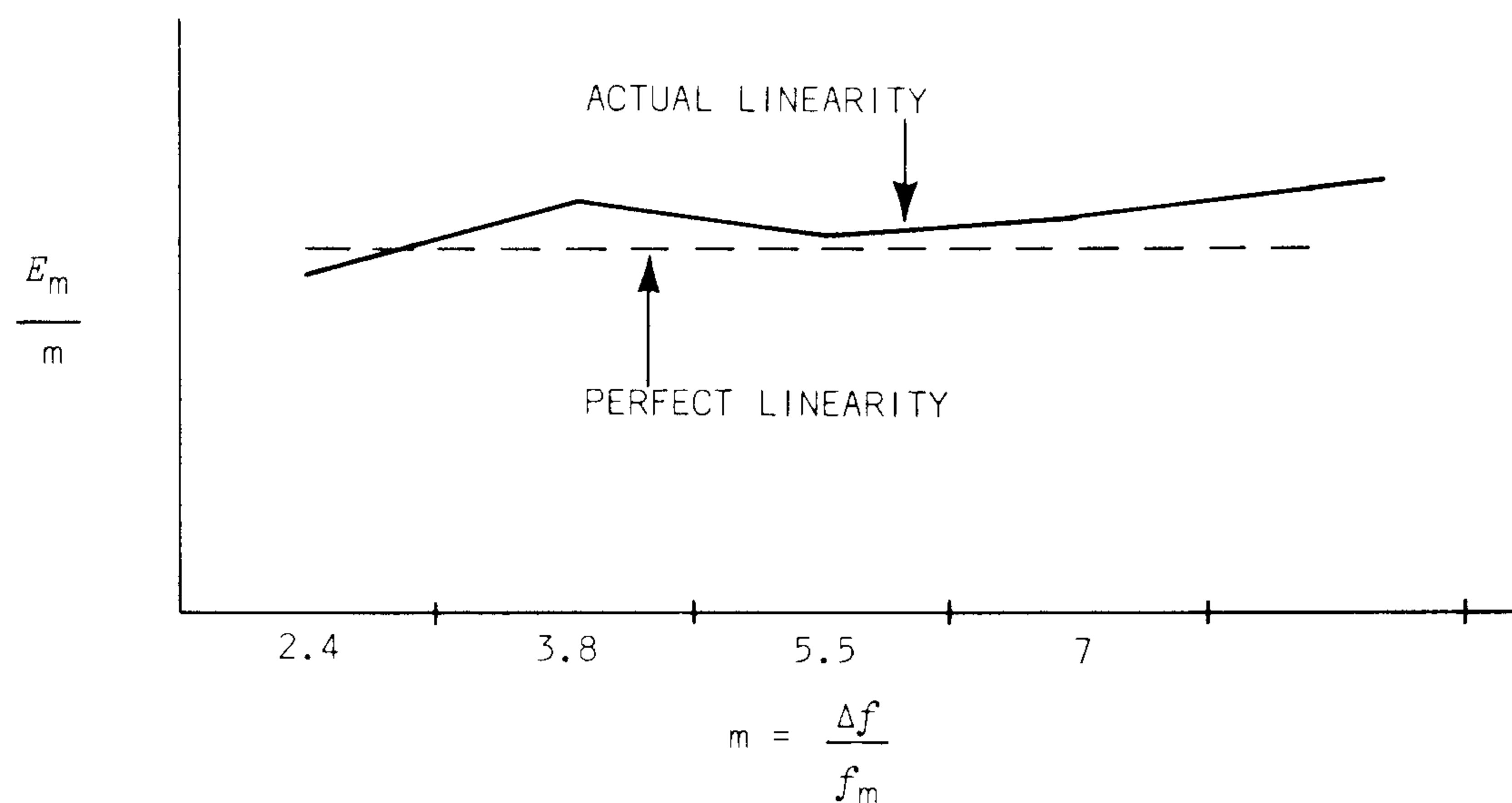
Fig. 8-5. Graphic display of deviation linearity.
