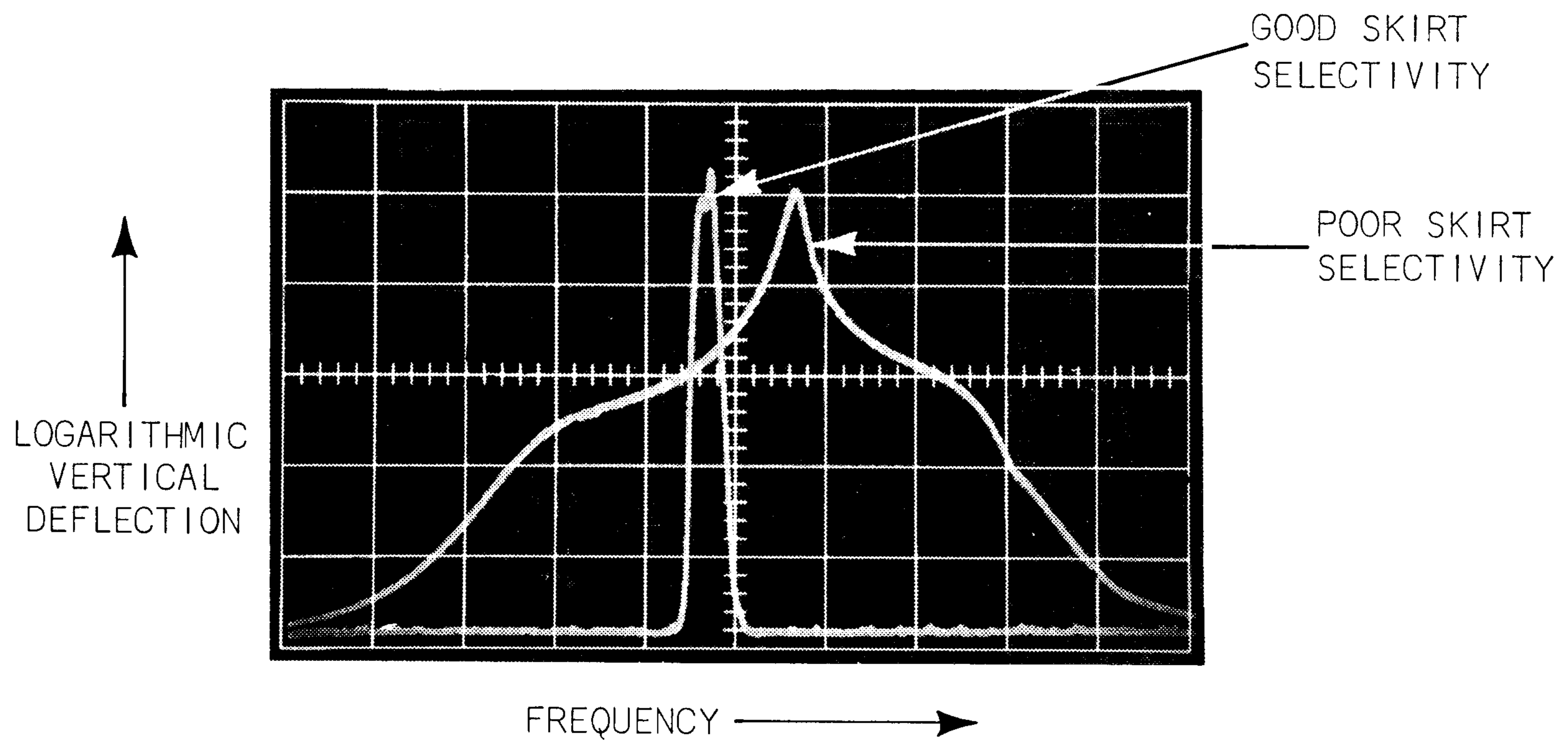
Fig. 3-4. Skirt selectivity.
