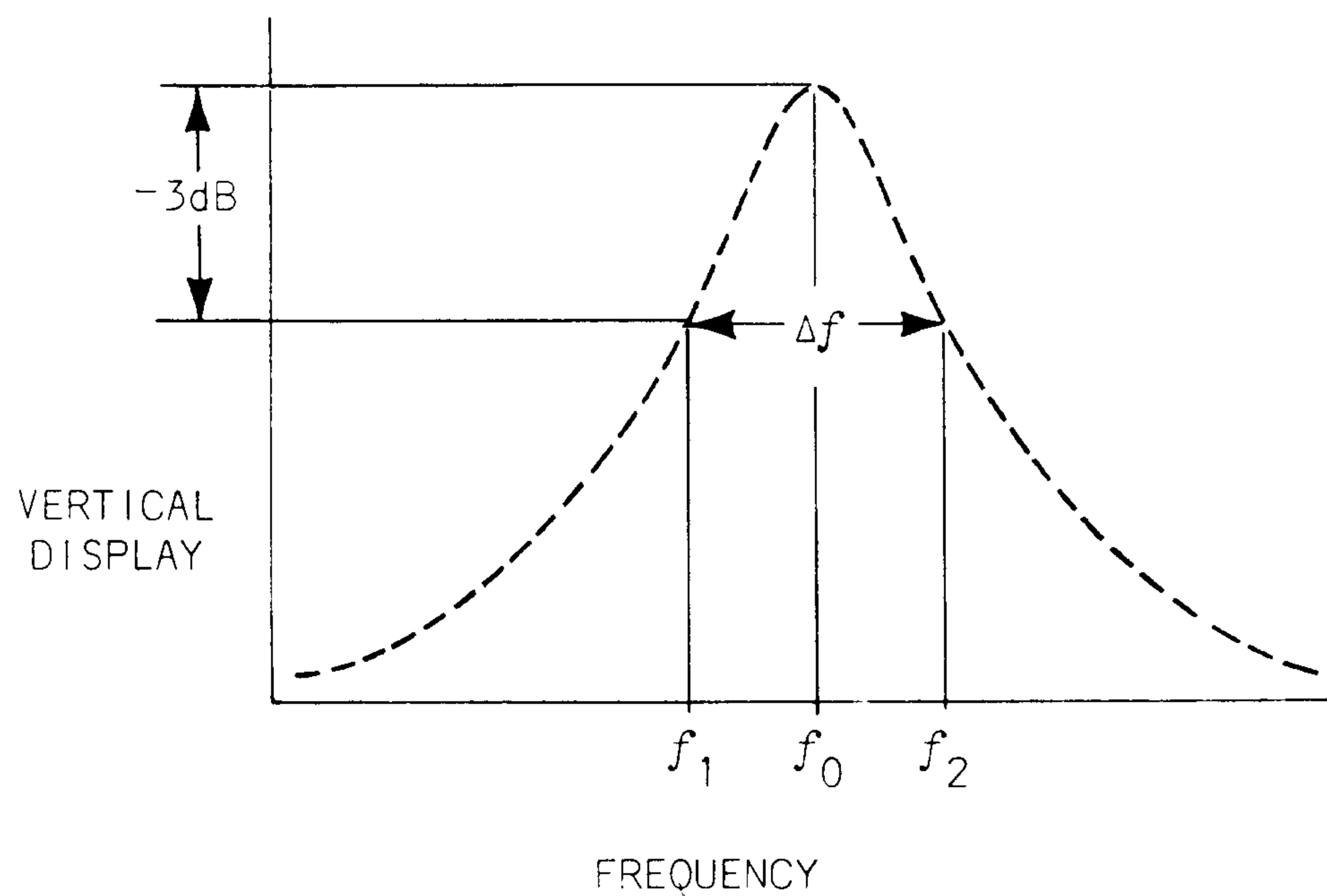
BROKEN LINES INDICATE LOCUS OF SIGNAL AMPLITUDE AS FREQUENCY IS VARIED THROUGH CAVITY RESONANCE
