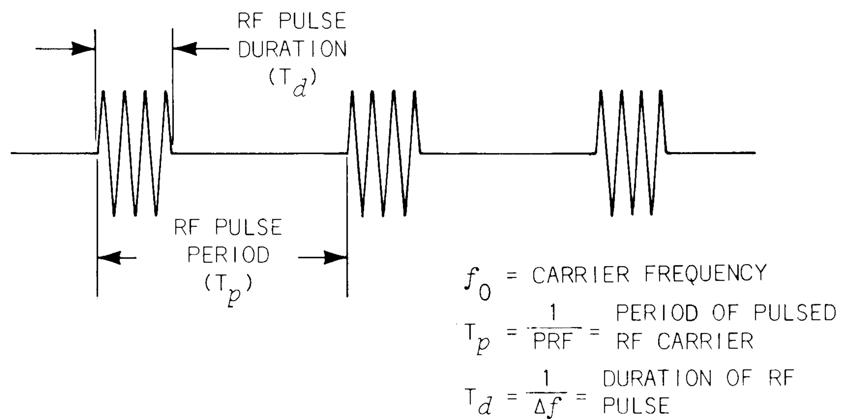
Fig. 2-5. Pulsed RF carrier in the time domain.
