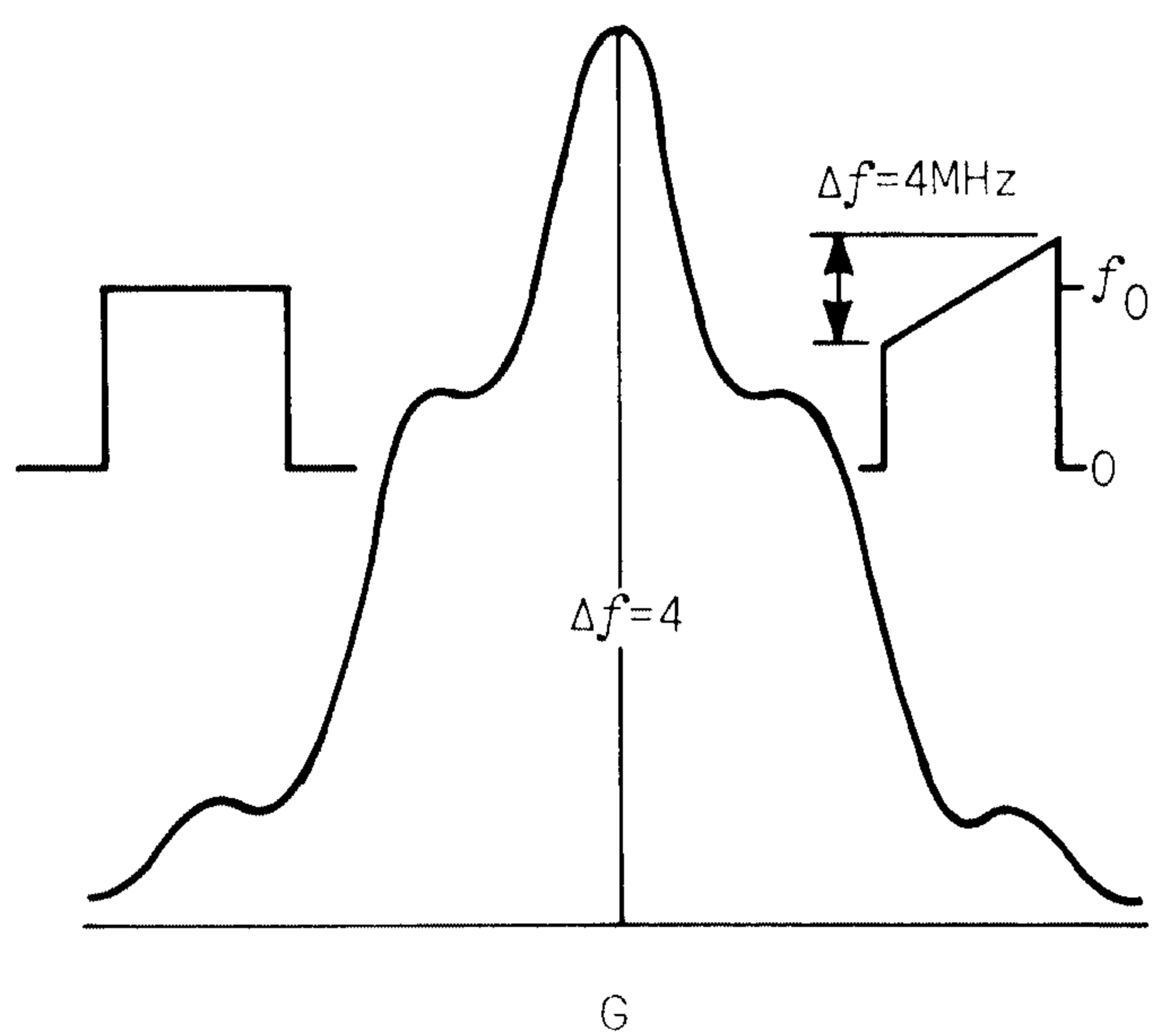
Fig. 10-5. Incidental AM and FM.
