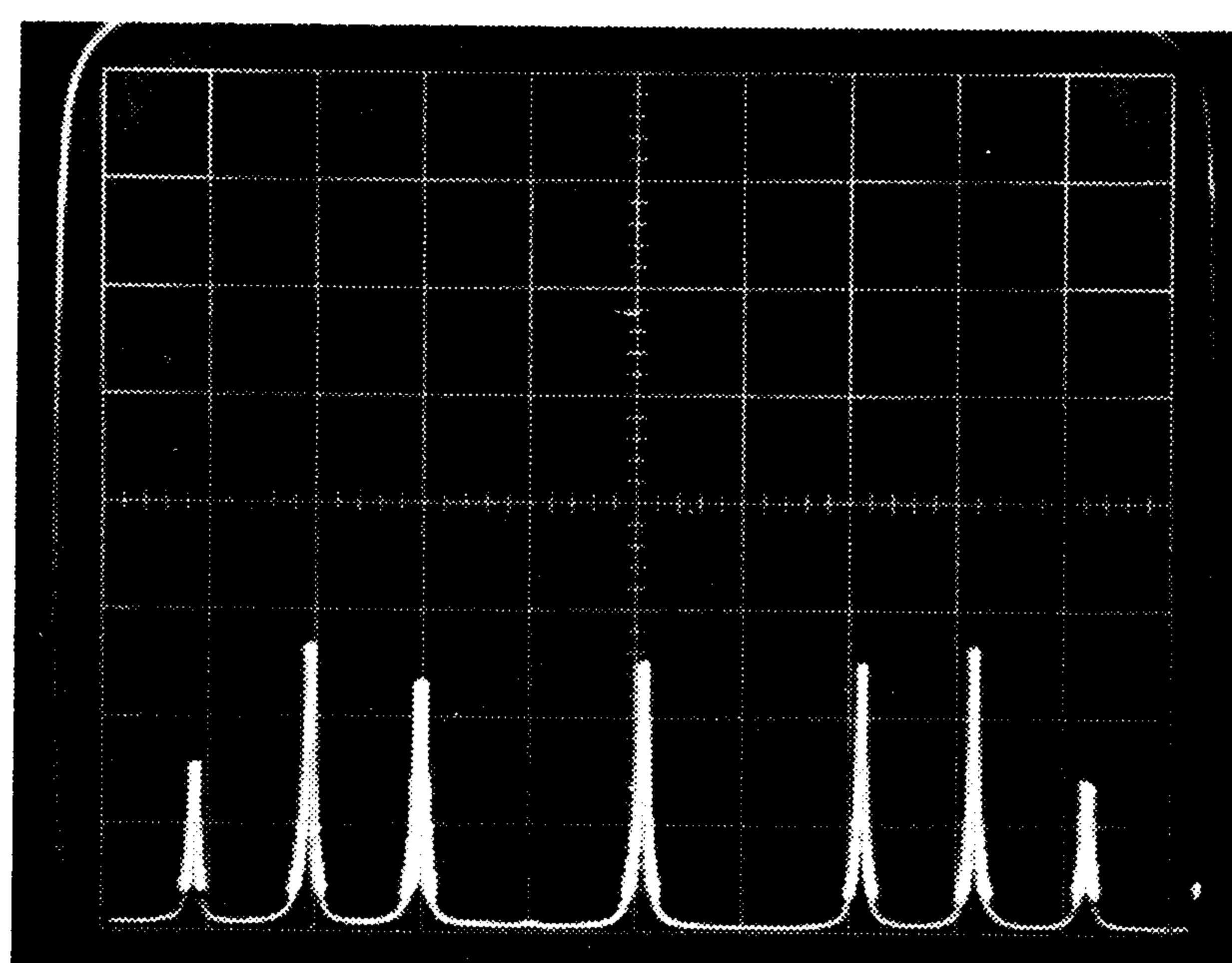
(B) FIRST SIDEBAND NULLS
