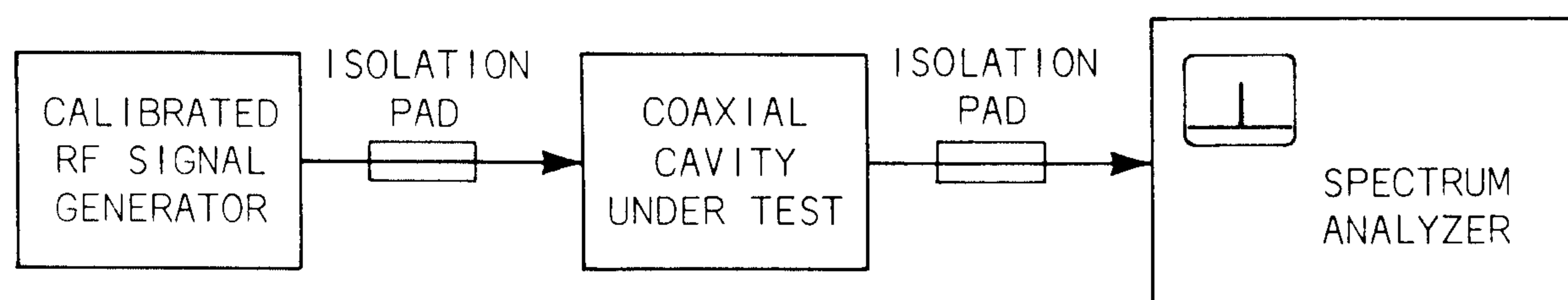
Q MEASUREMENT METHOD FOR TRANSMISSION-TYPE CAVITIES
