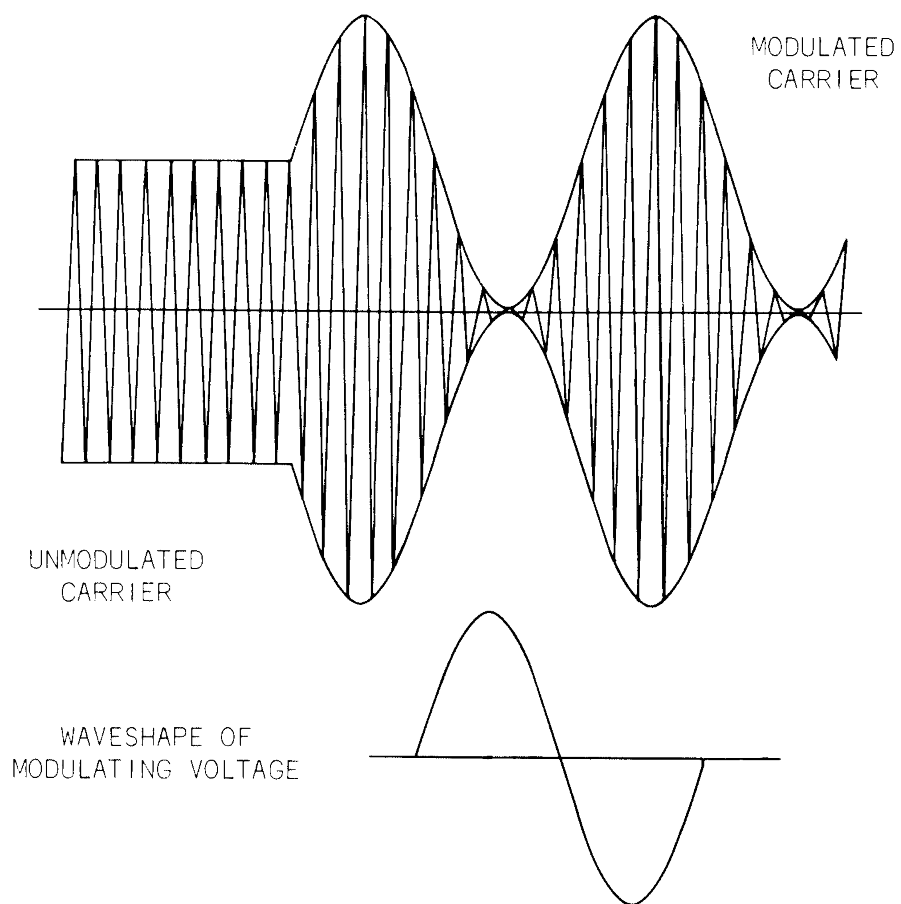
Fig. 2-2. Time domain display of 100% modulated RF carrier.
