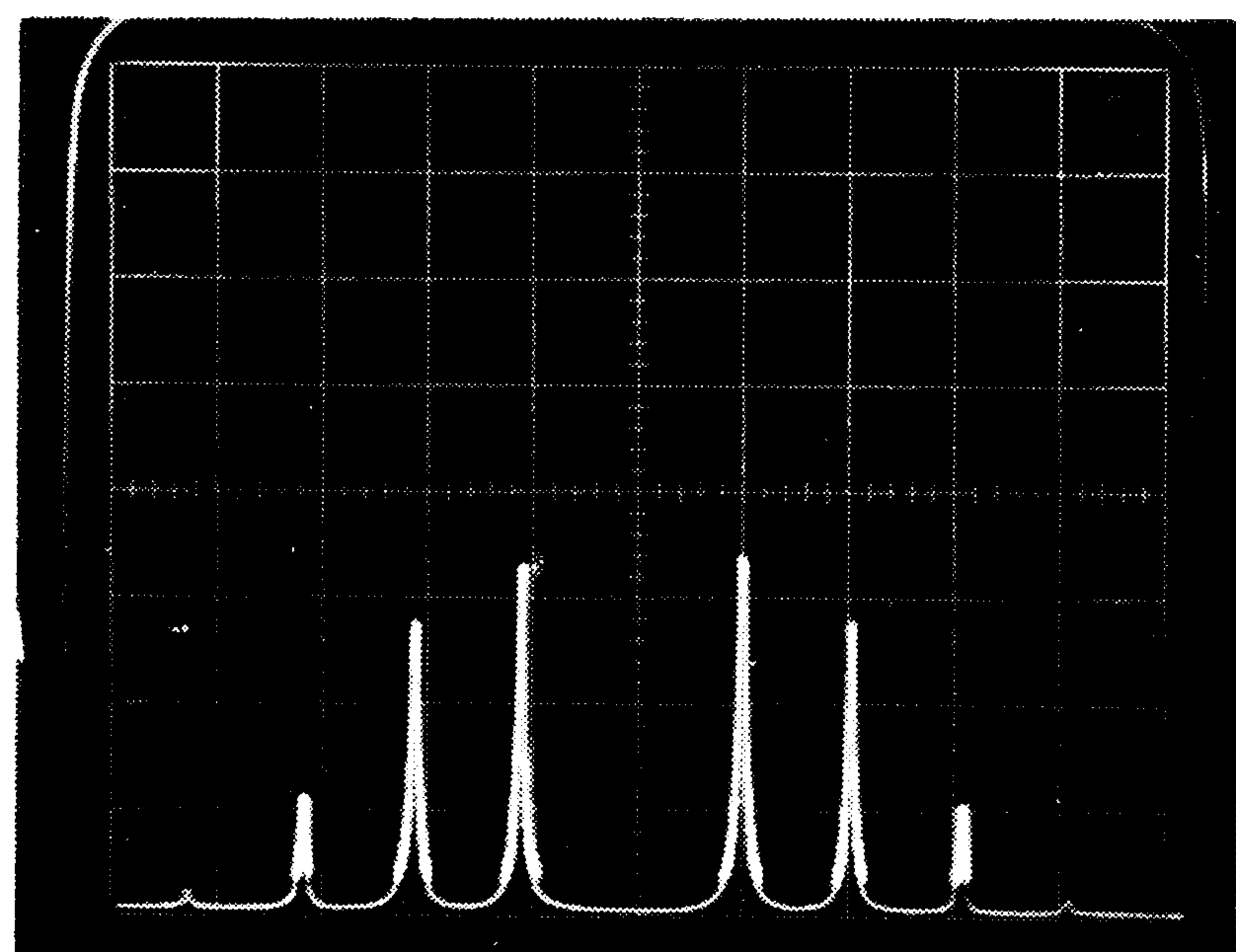
(A) CARRIER NULL
