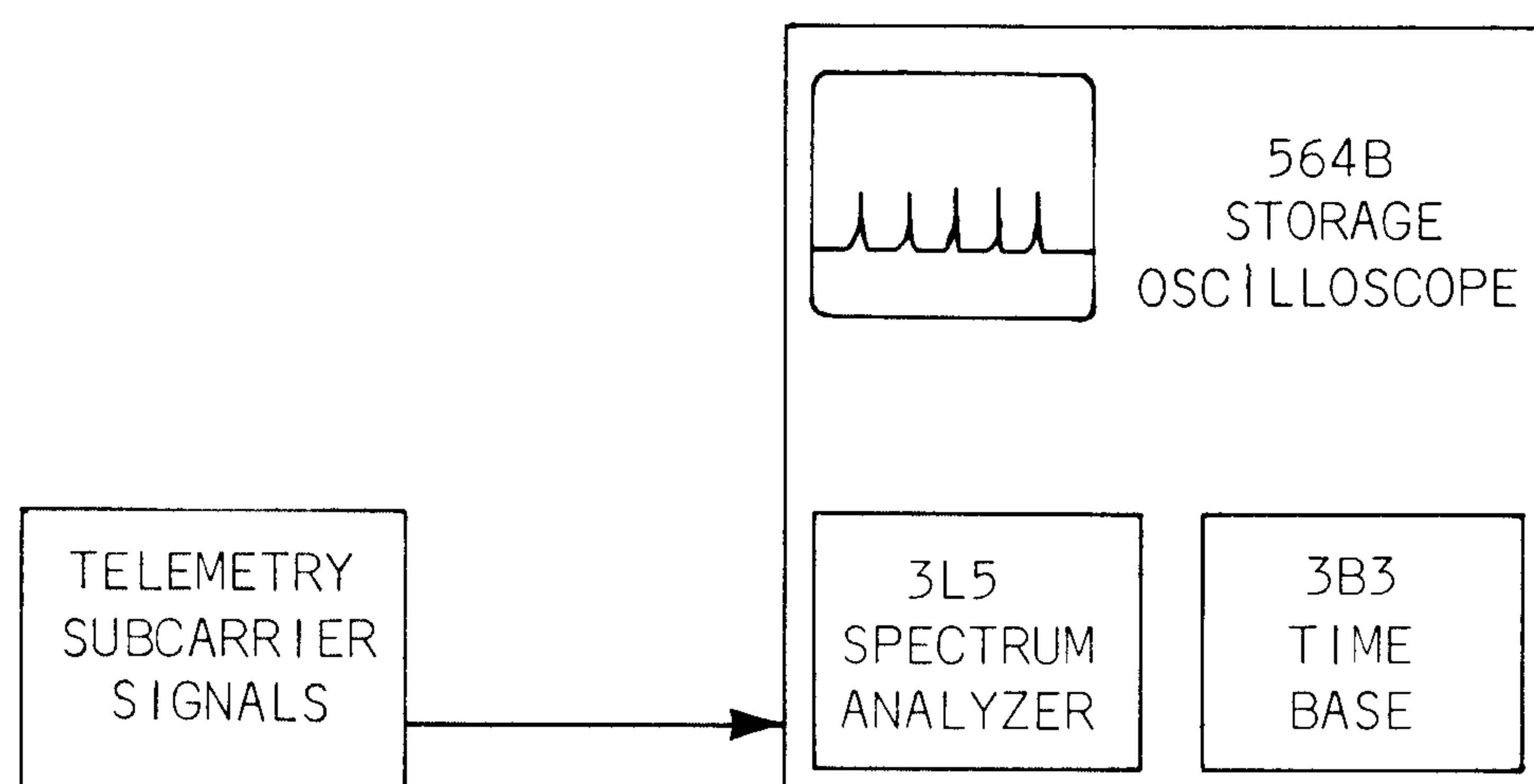
Fig. 7-3. Illustration of method of displaying telemetry subcarriers.
