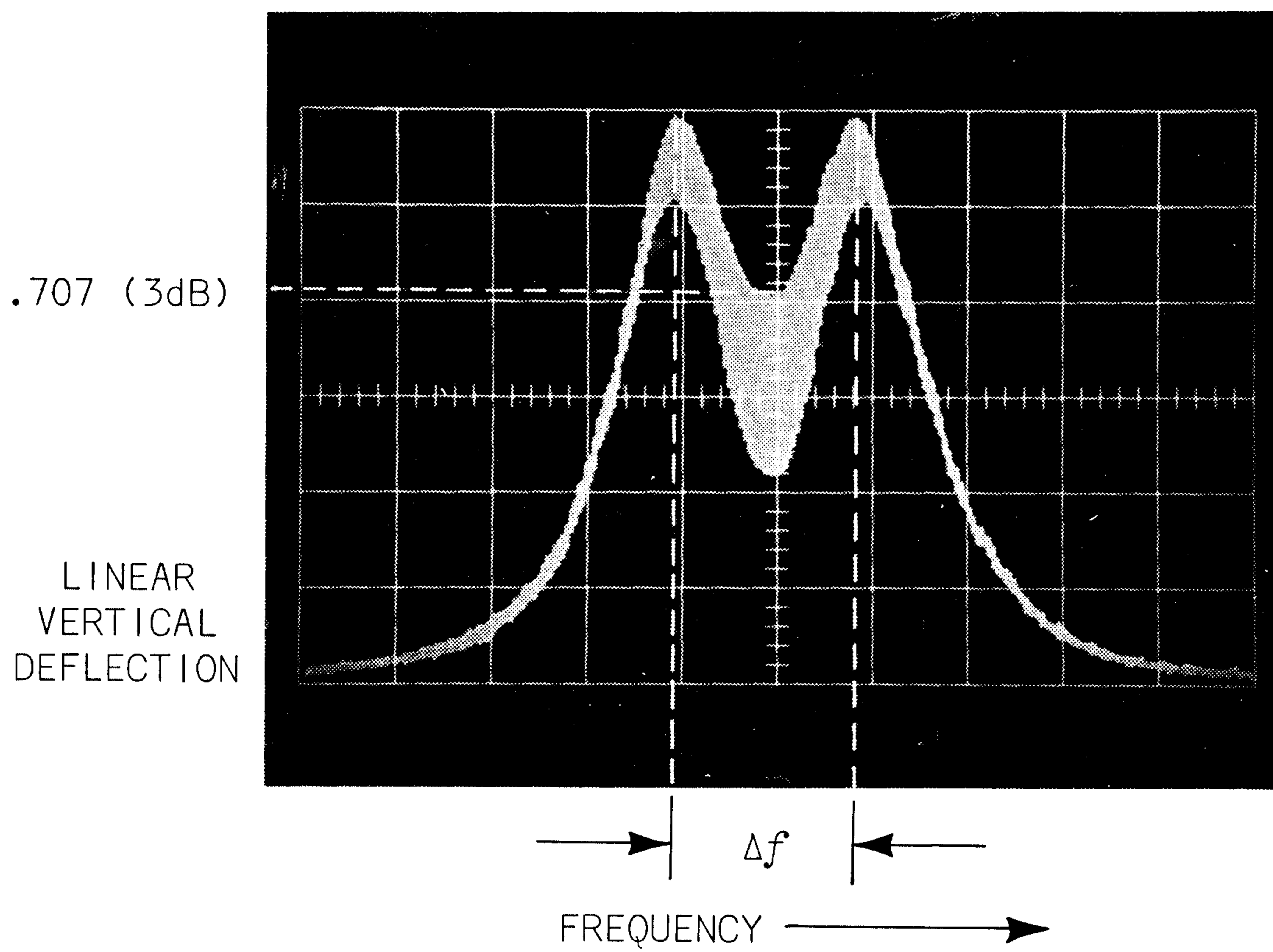
(A) RESOLUTION IS \Delta f
