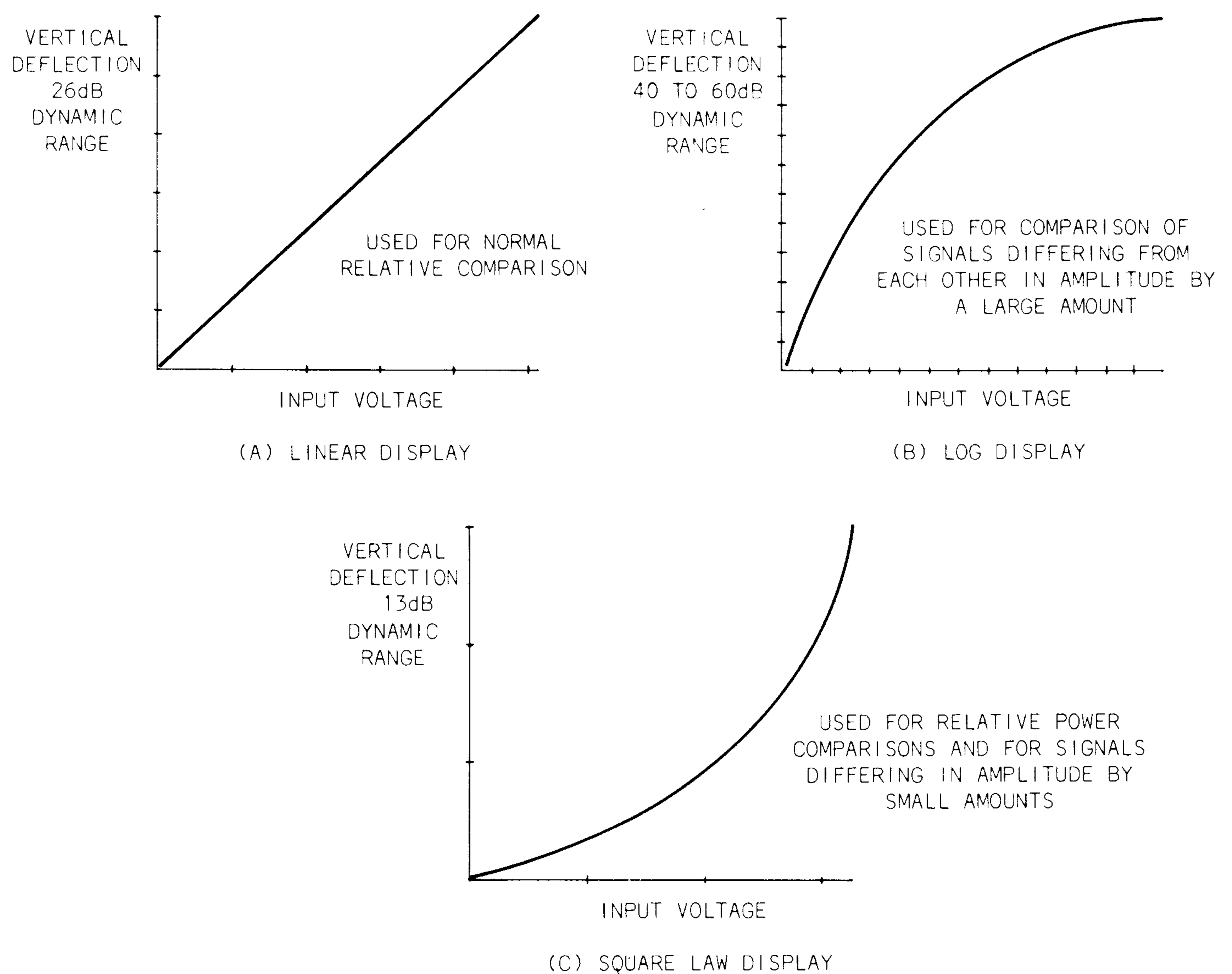
Fig. 3-1. Dynamic range.
