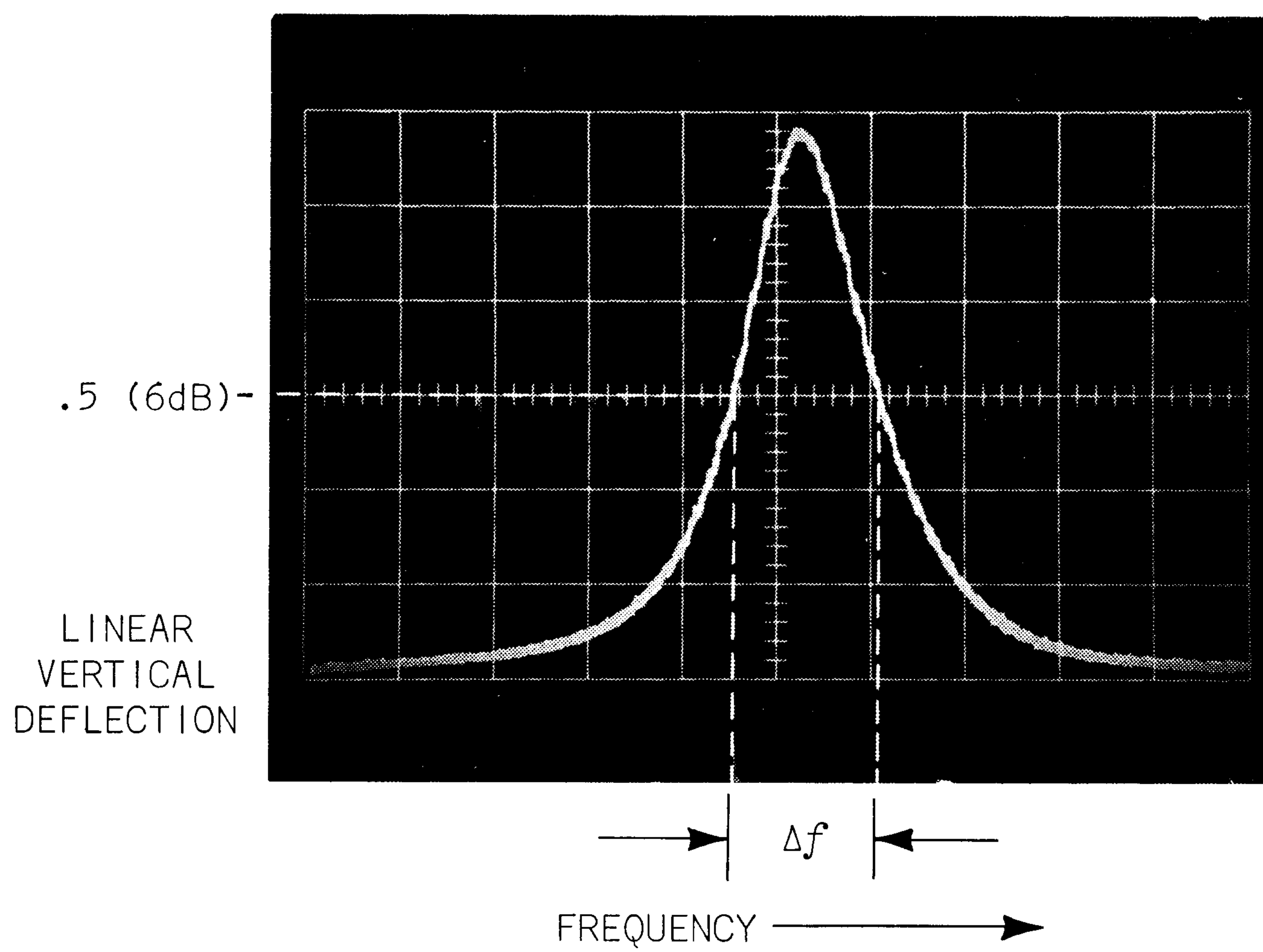
(B) ALTERNATE DEFINITION OF RESOLUTION ( \Delta f )
