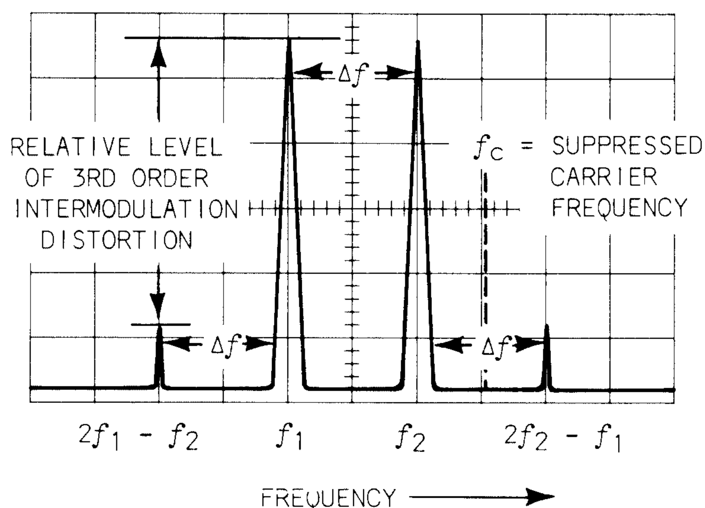
Fig. 9-4. Intermodulation or signal-to-distortion measurement.
