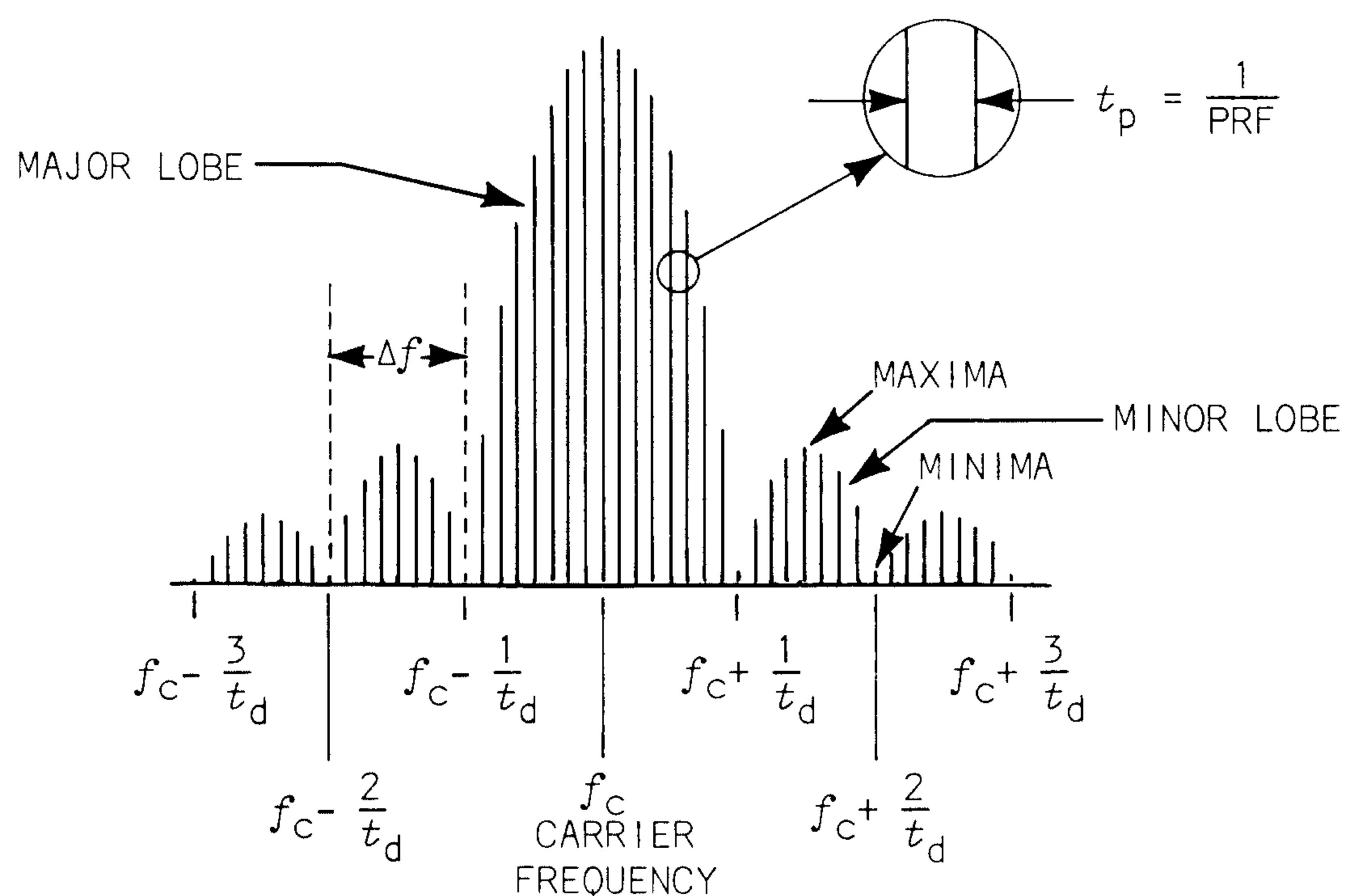
Fig. 10-2. Pulsed RF spectrum display.
