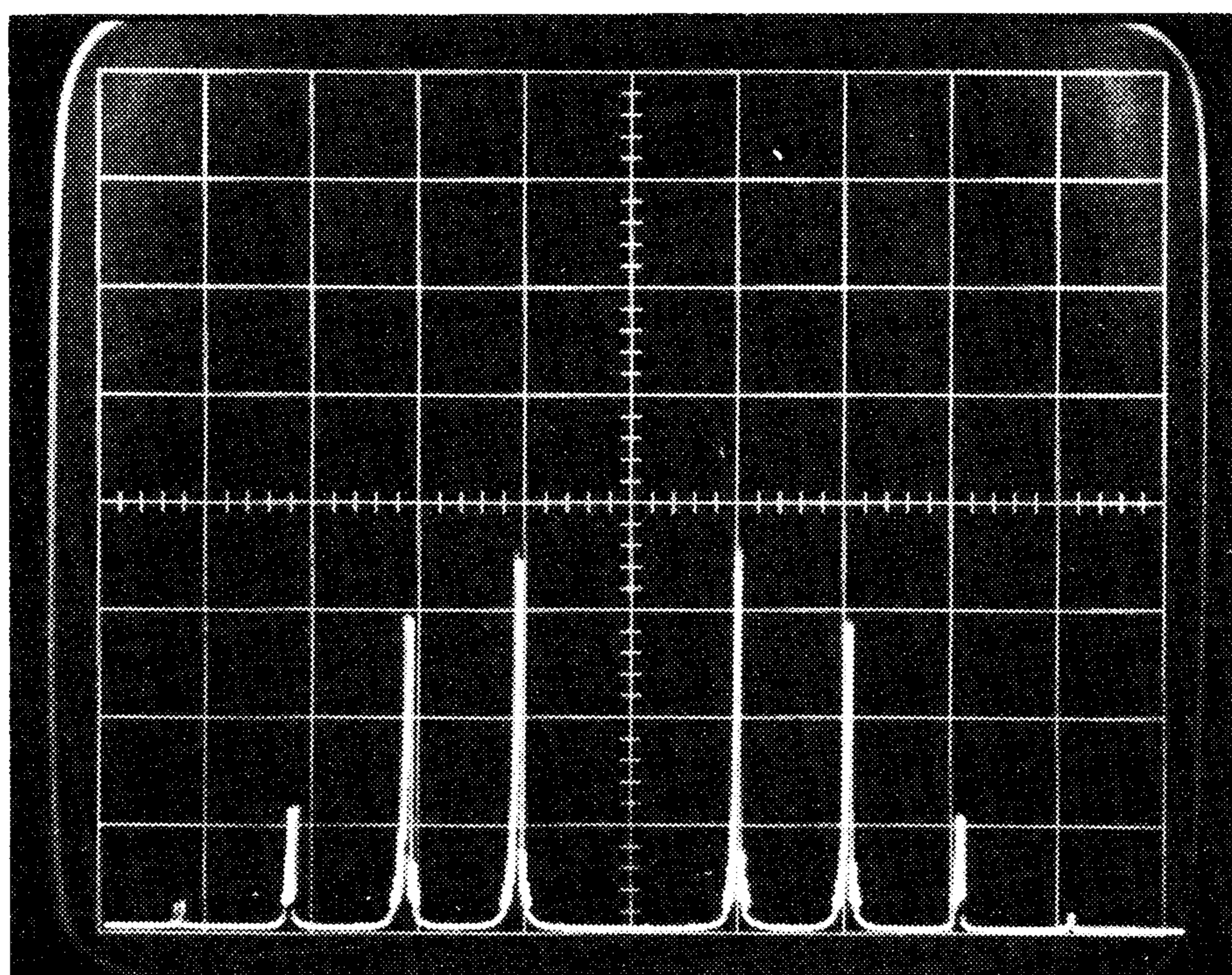
(C) CARRIER FREQUENCY AT FIRST NULL -- MODULATION INDEX OF 2.4, SEE FIG. 8-4
