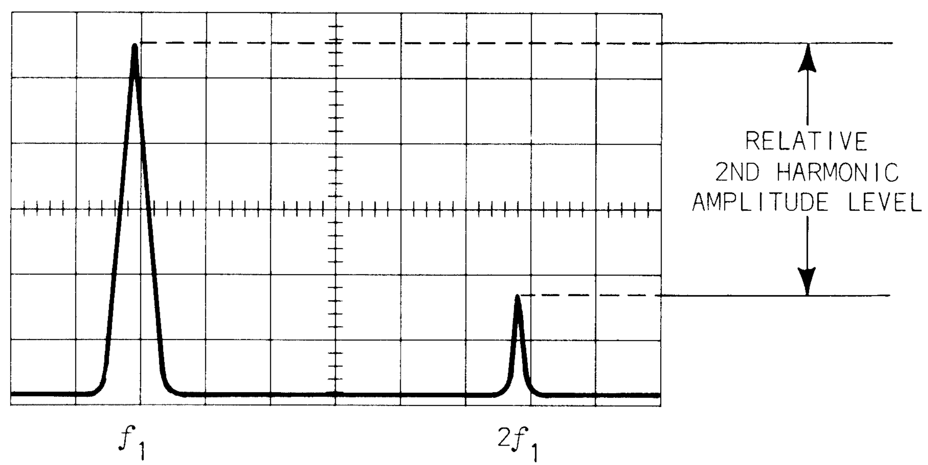
Fig. 6-7. Display shown for relative harmonic measurement.
