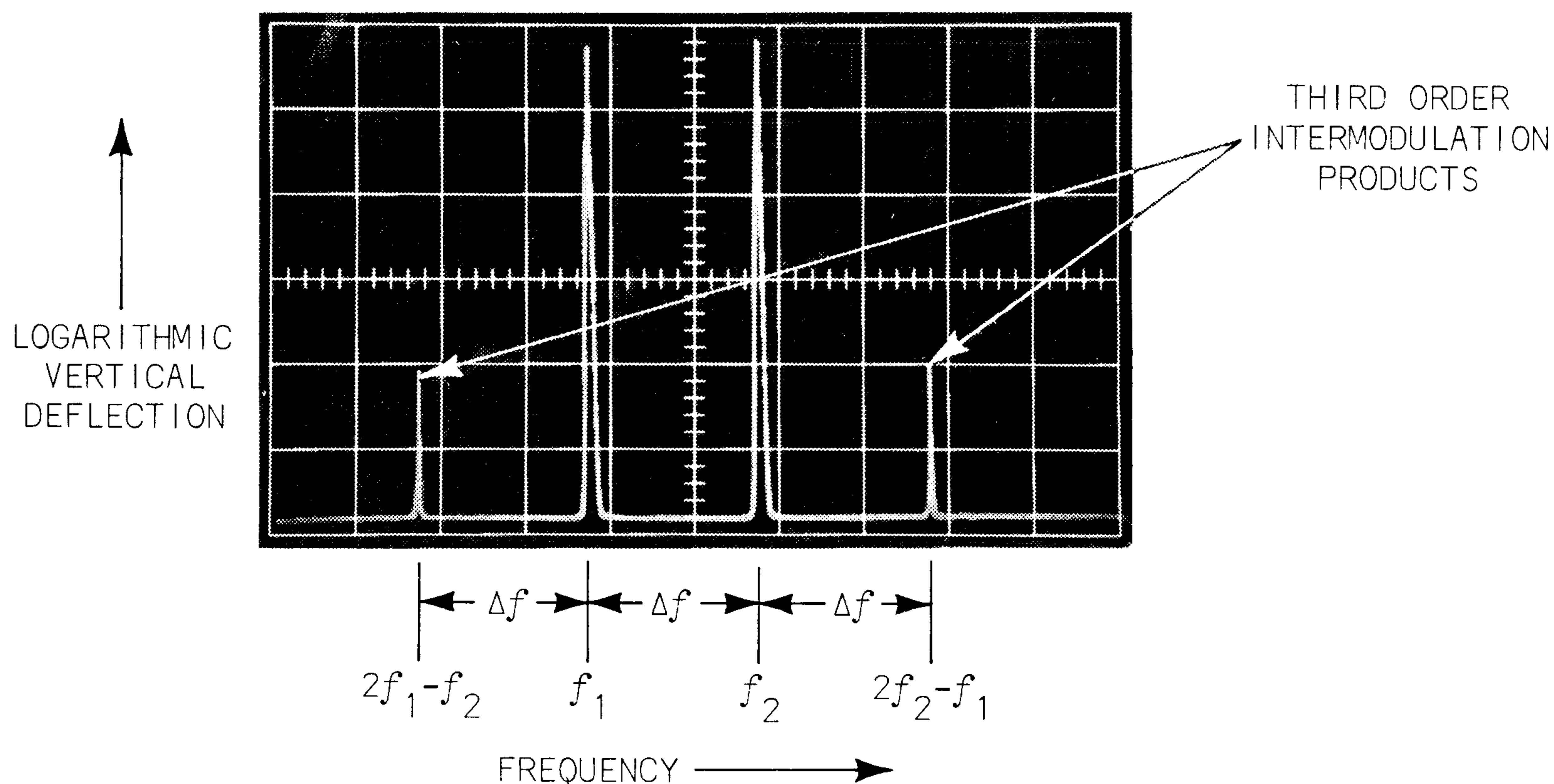
Fig. 3-5. Intermodulation.
