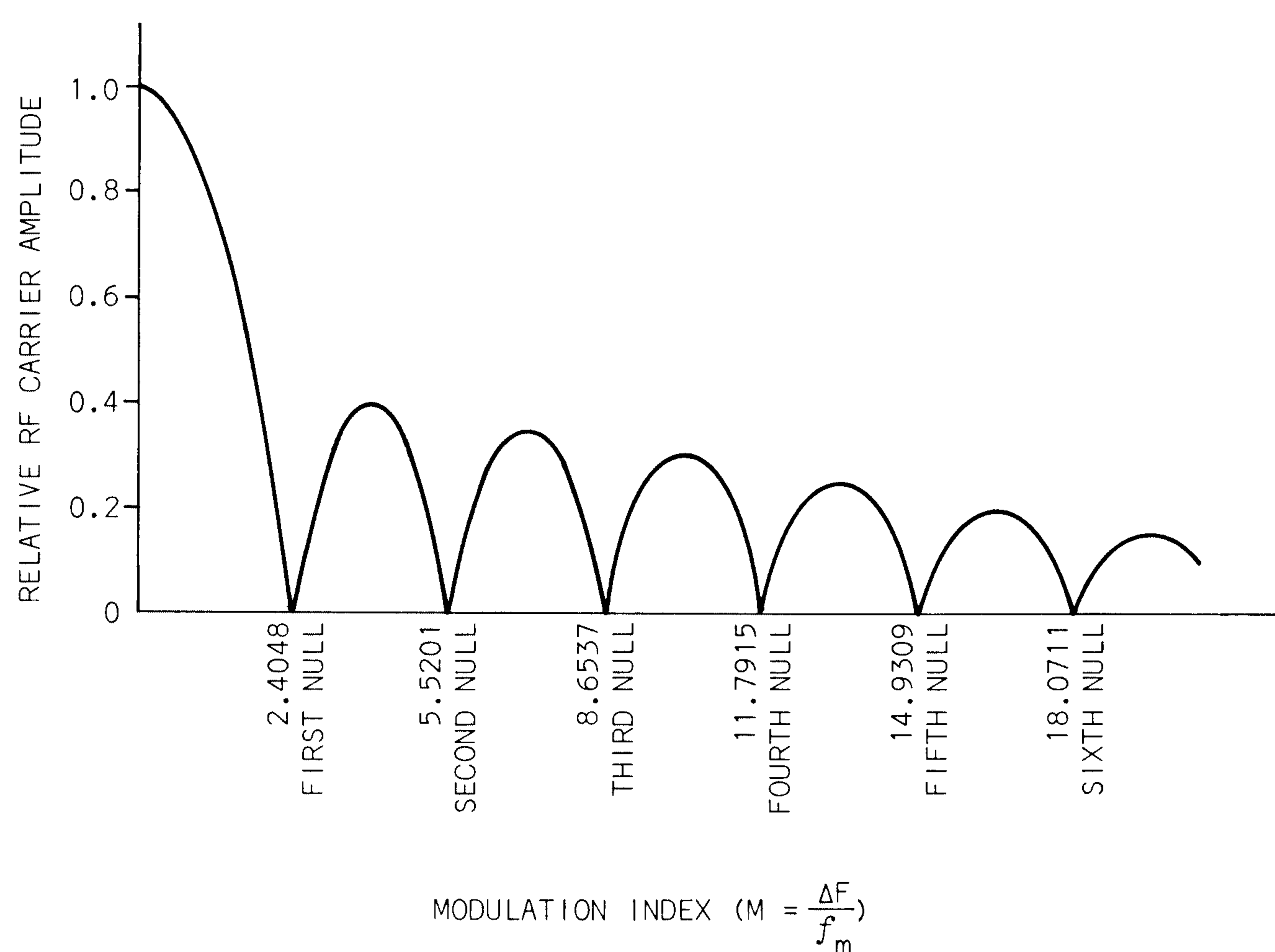
Fig. 8-4. Carrier null versus modulation index.
