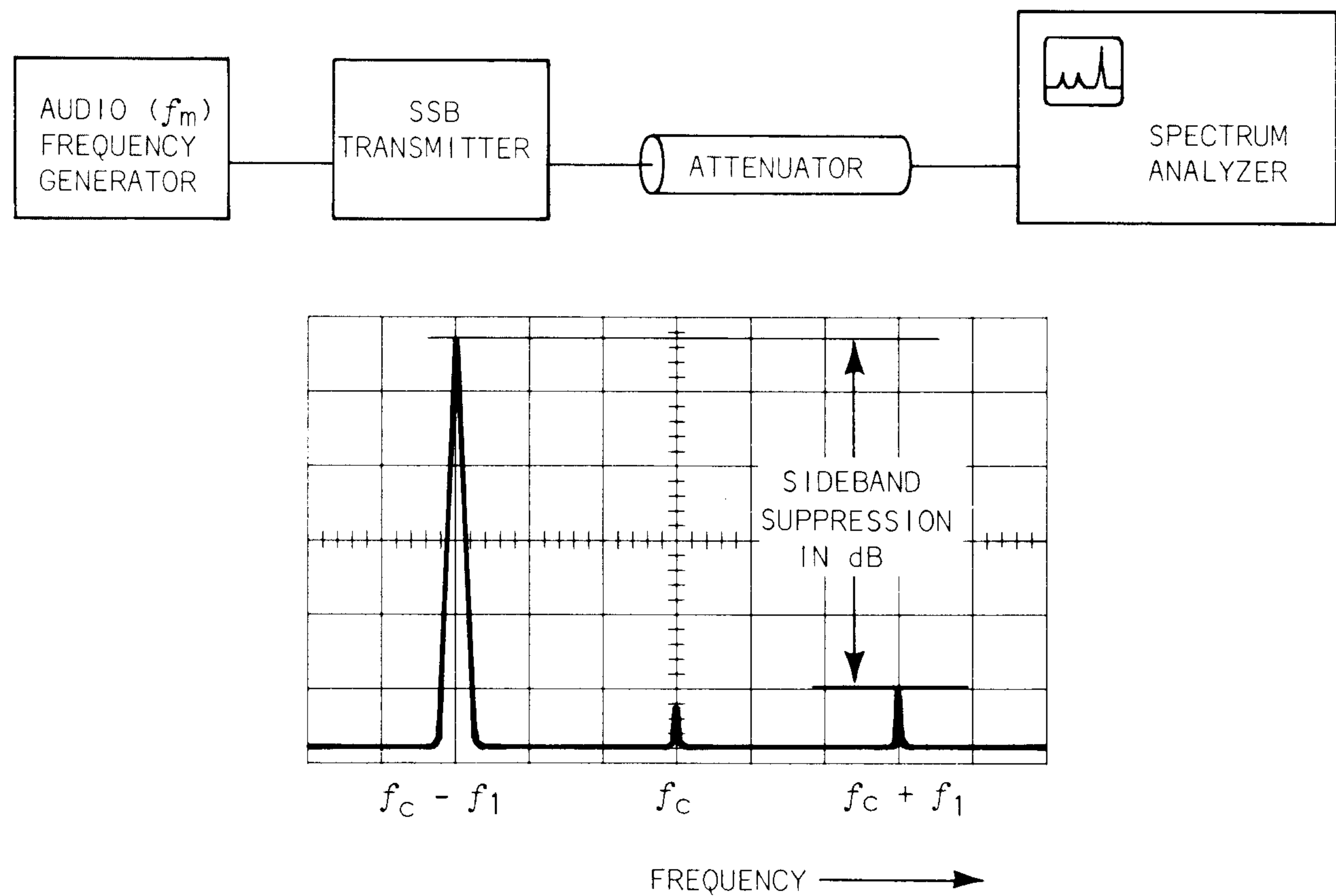
Fig. 9-2. Sideband suppression measurement.
