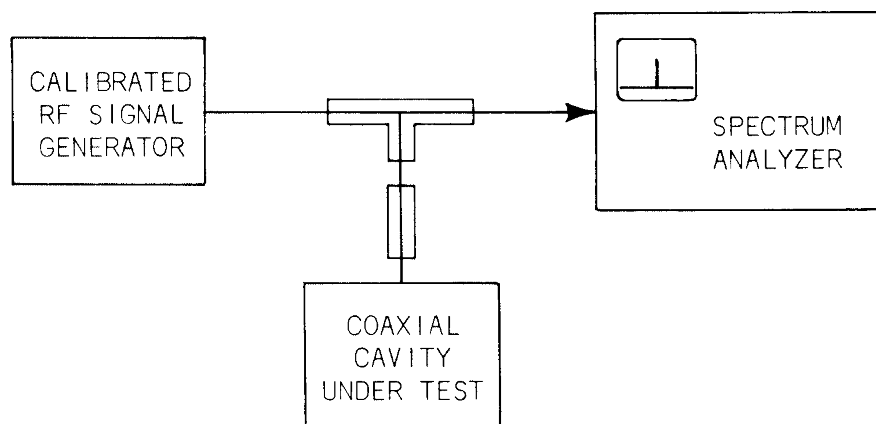
Q MEASUREMENT METHOD FOR ABSORPTION-TYPE CAVITIES
