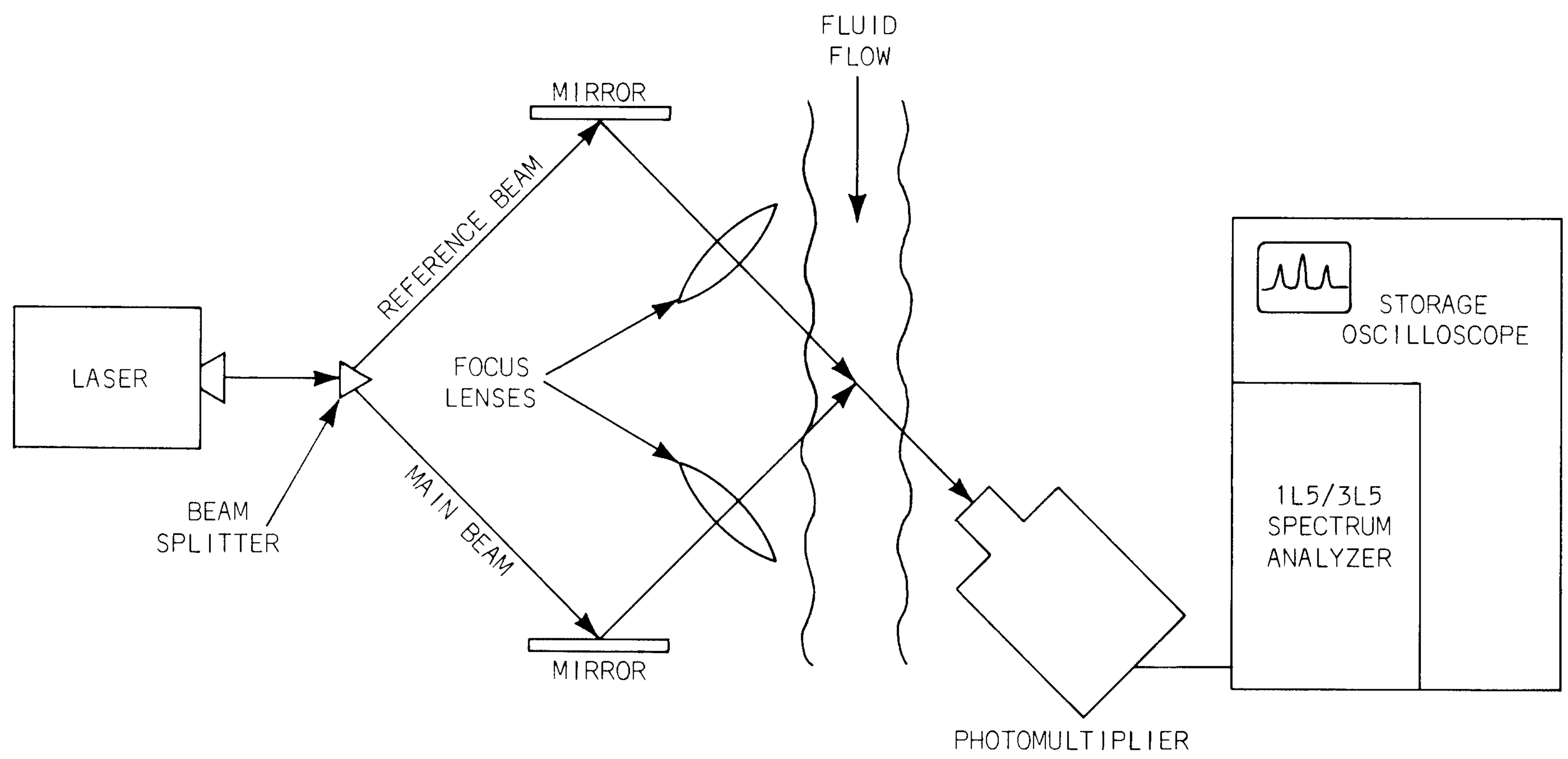
Fig. 12-1. Method of performing fluid velocity measurement.
