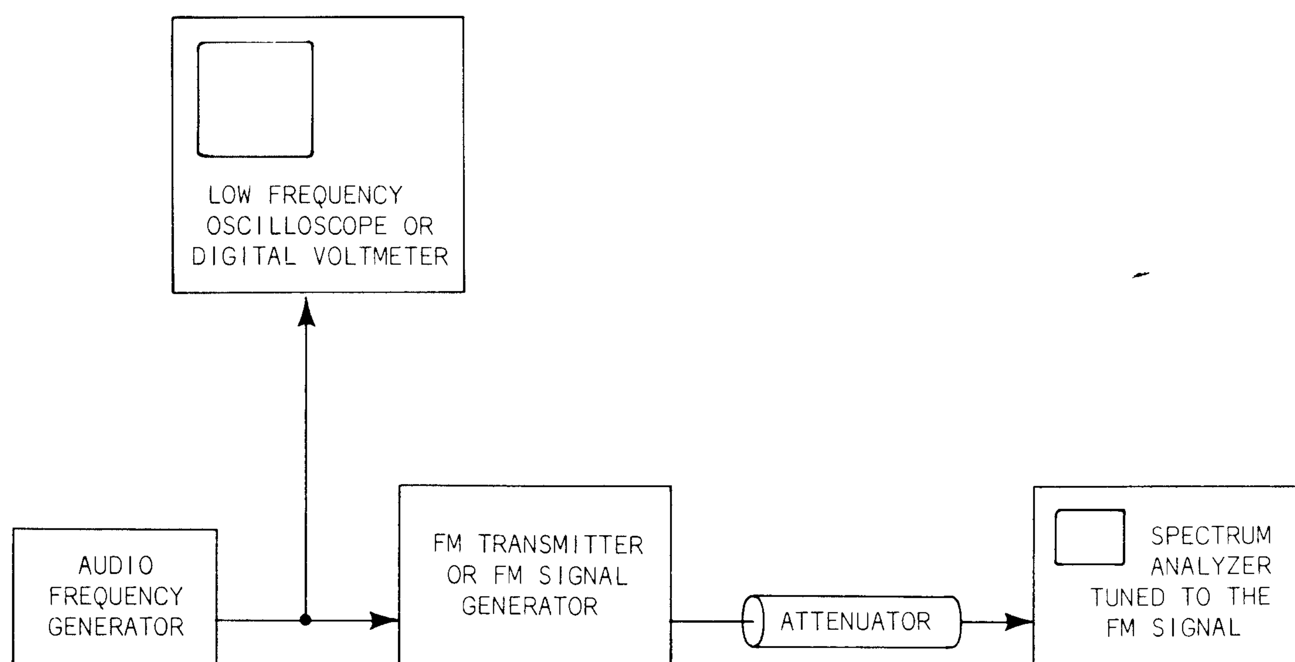
Fig. 8-6. FM deviation linearity measurement.
