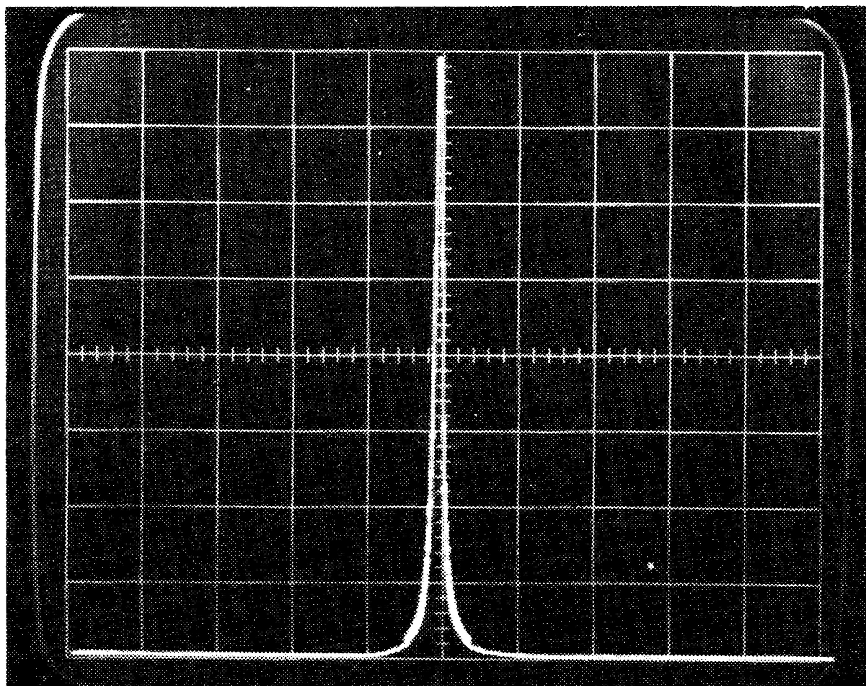
(A) UNMODULATED FM CARRIER AS DISPLAYED ON A TEKTRONIX TYPE 491 SPECTRUM ANALYZER
