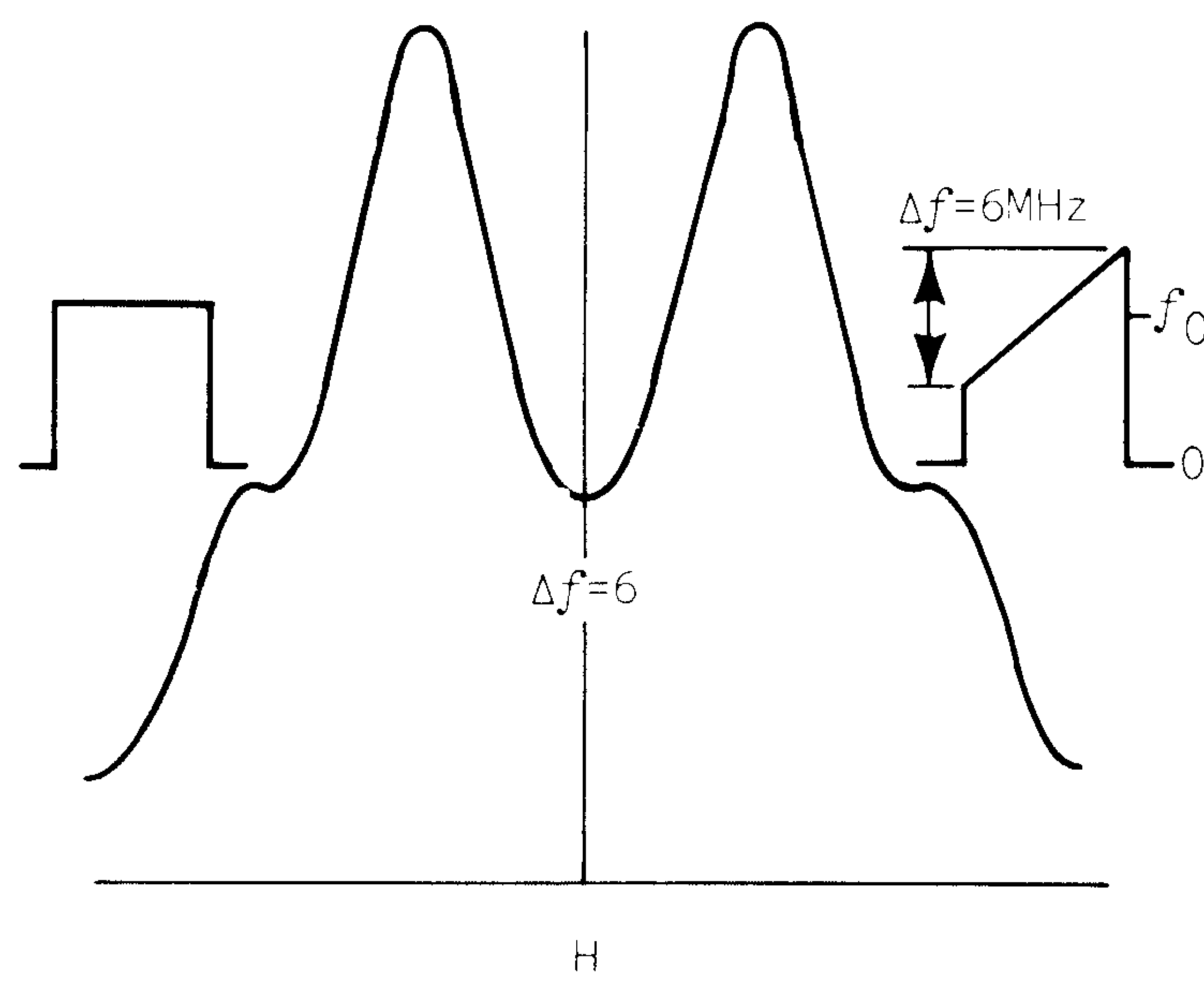
Fig. 2-8. Common RF spectra.
