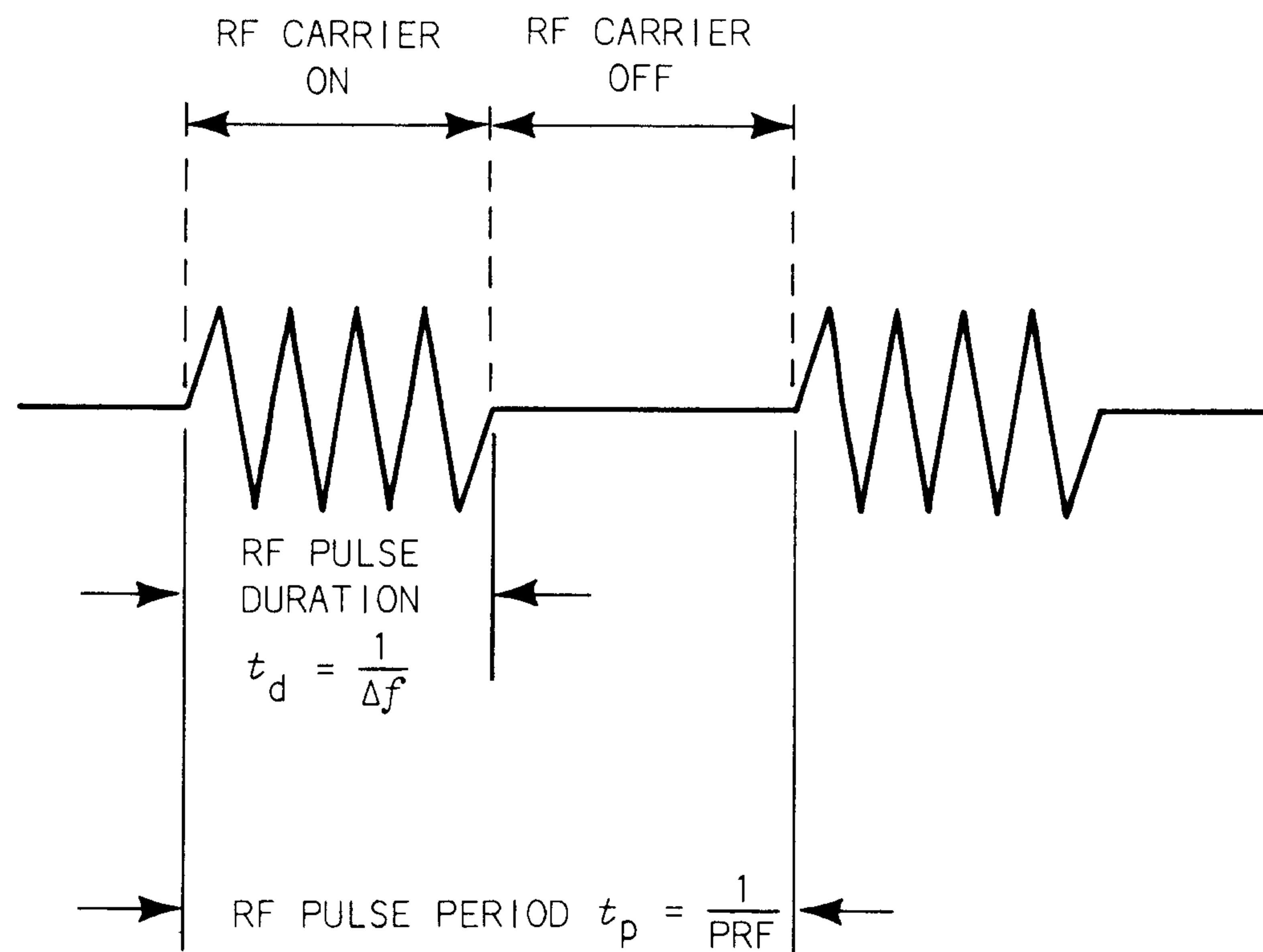
Fig. 10-3. Pulsed RF signal.
