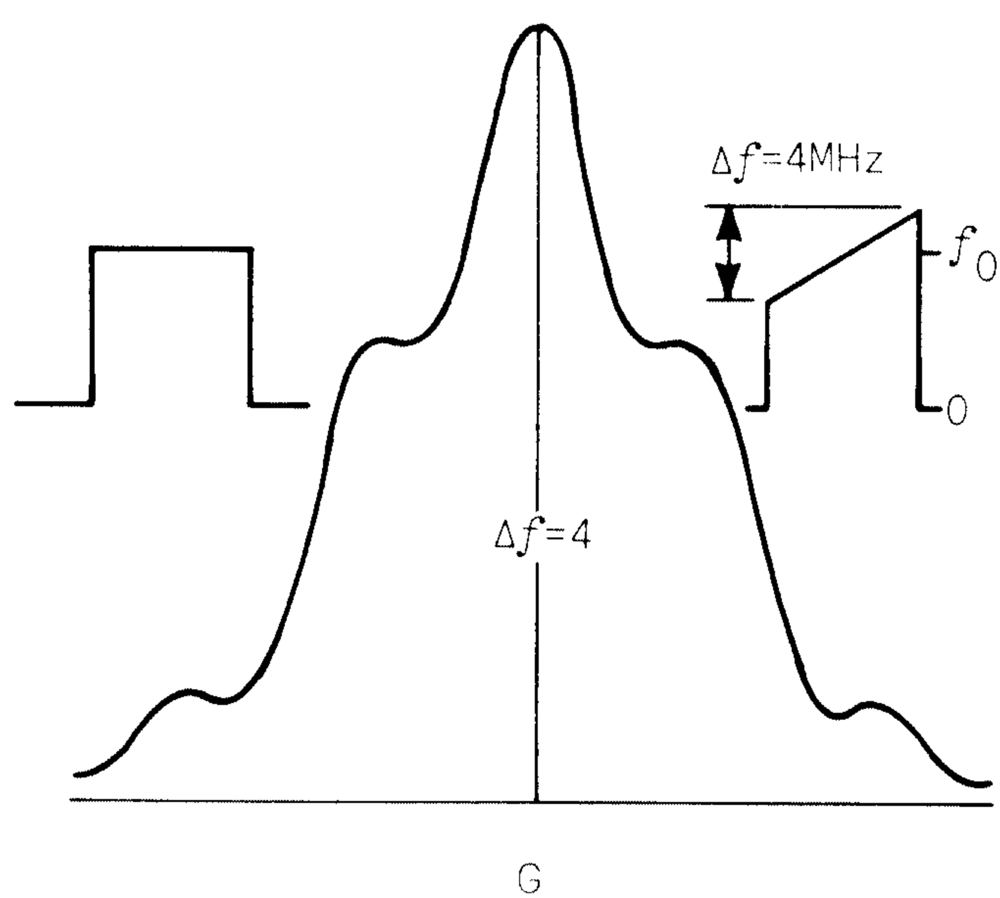
Fig. 2-8. Common RF spectra.
