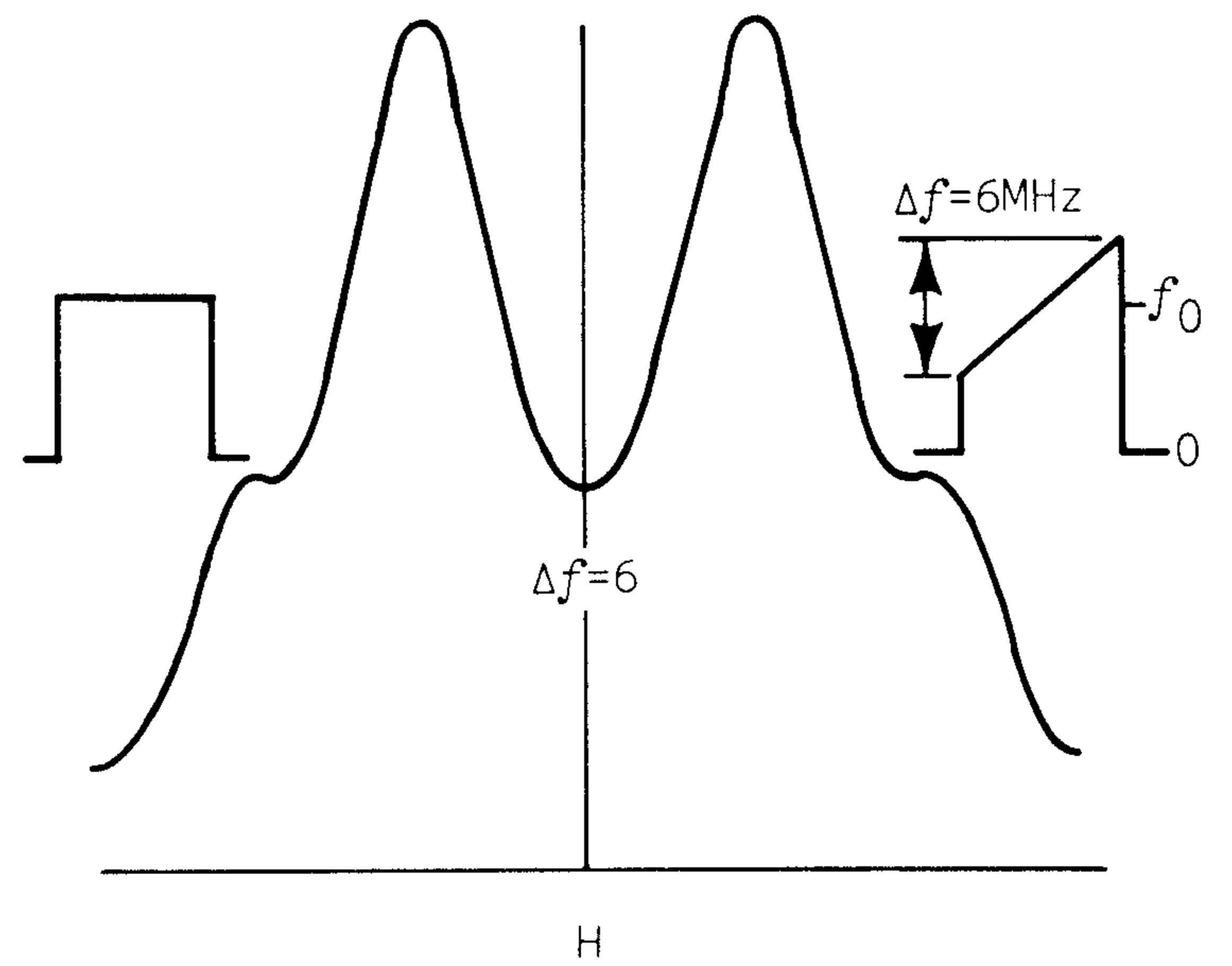
Fig. 10-5. Incidental AM and FM.
