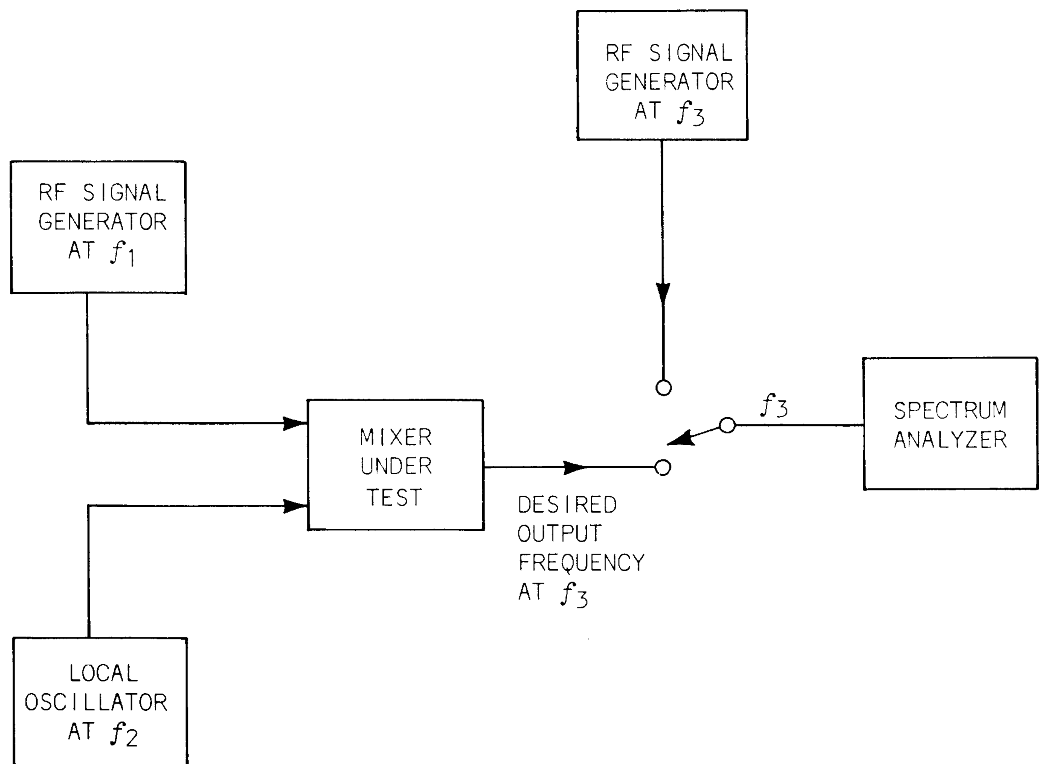
Fig. 6-9. Typical method for conversion loss measurement.
