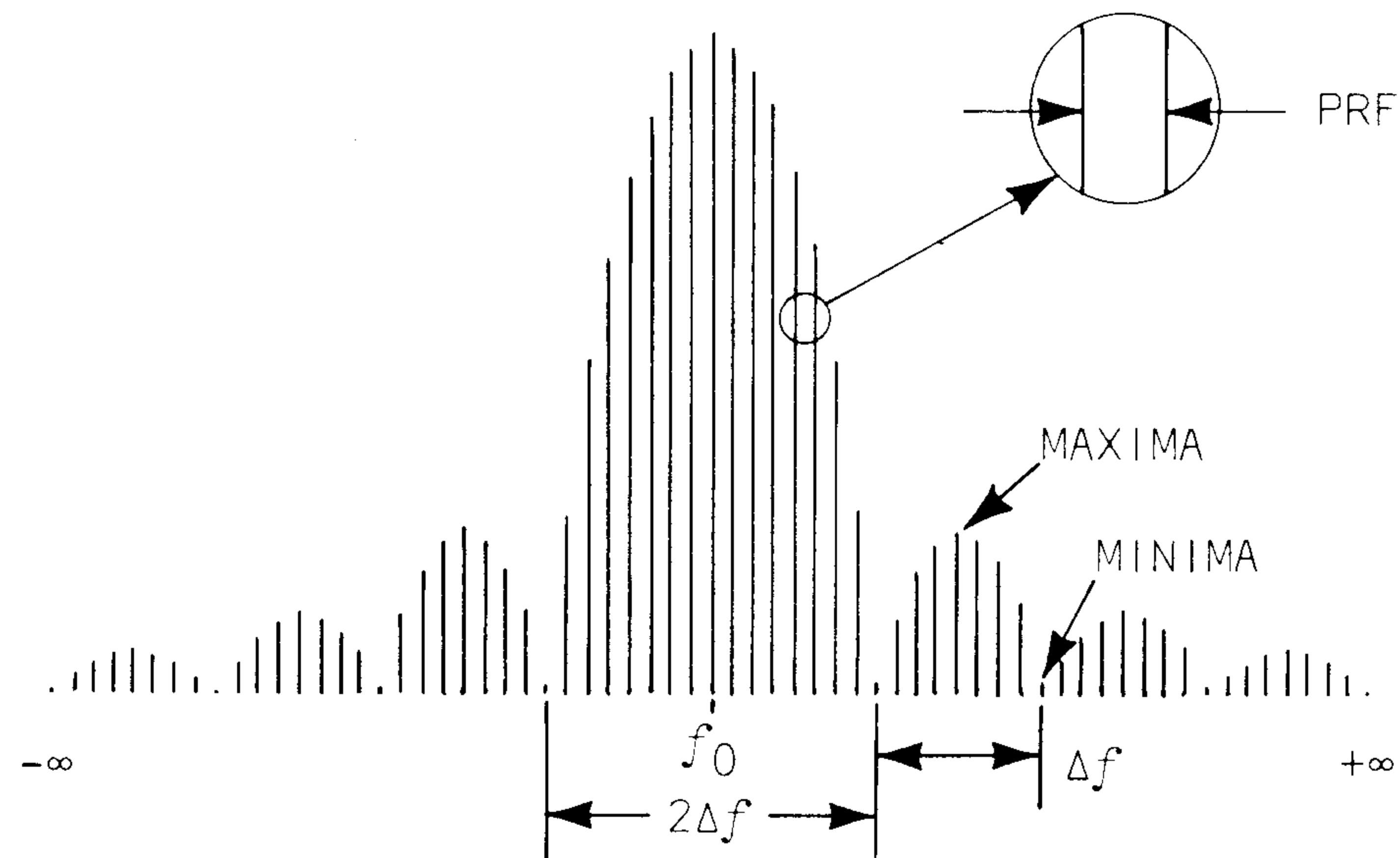
Fig. 2-6. Illustration of a pulsed RF spectrum ( \frac{\sin x}{x} type) in the frequency domain.
