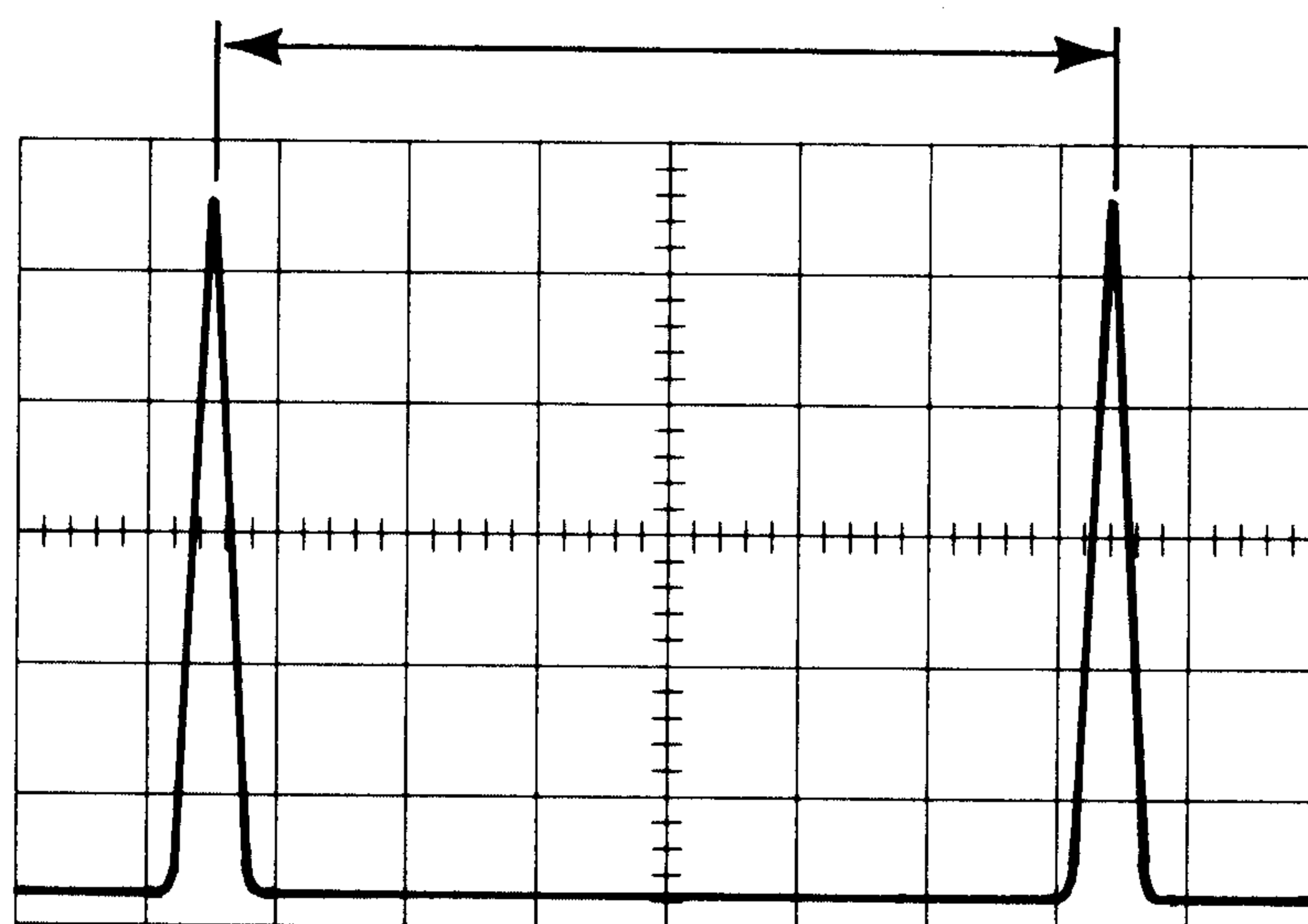
Fig. 10-4. Pulse period ( t_p = \frac{1}{\text{PRF}} ) measurement.
