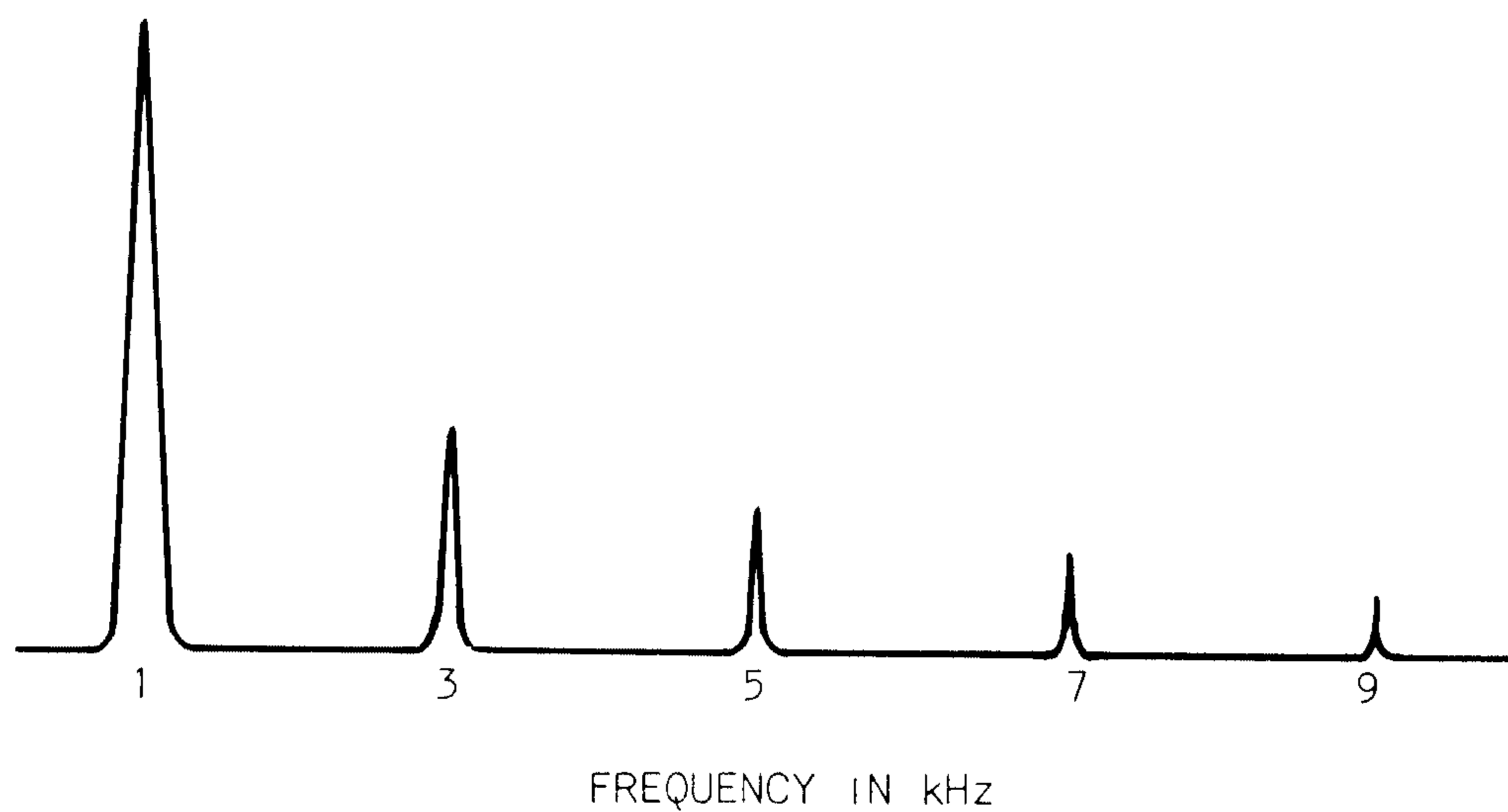
(B) FOURIER-SERIES FREQUENCY COMPONENTS
