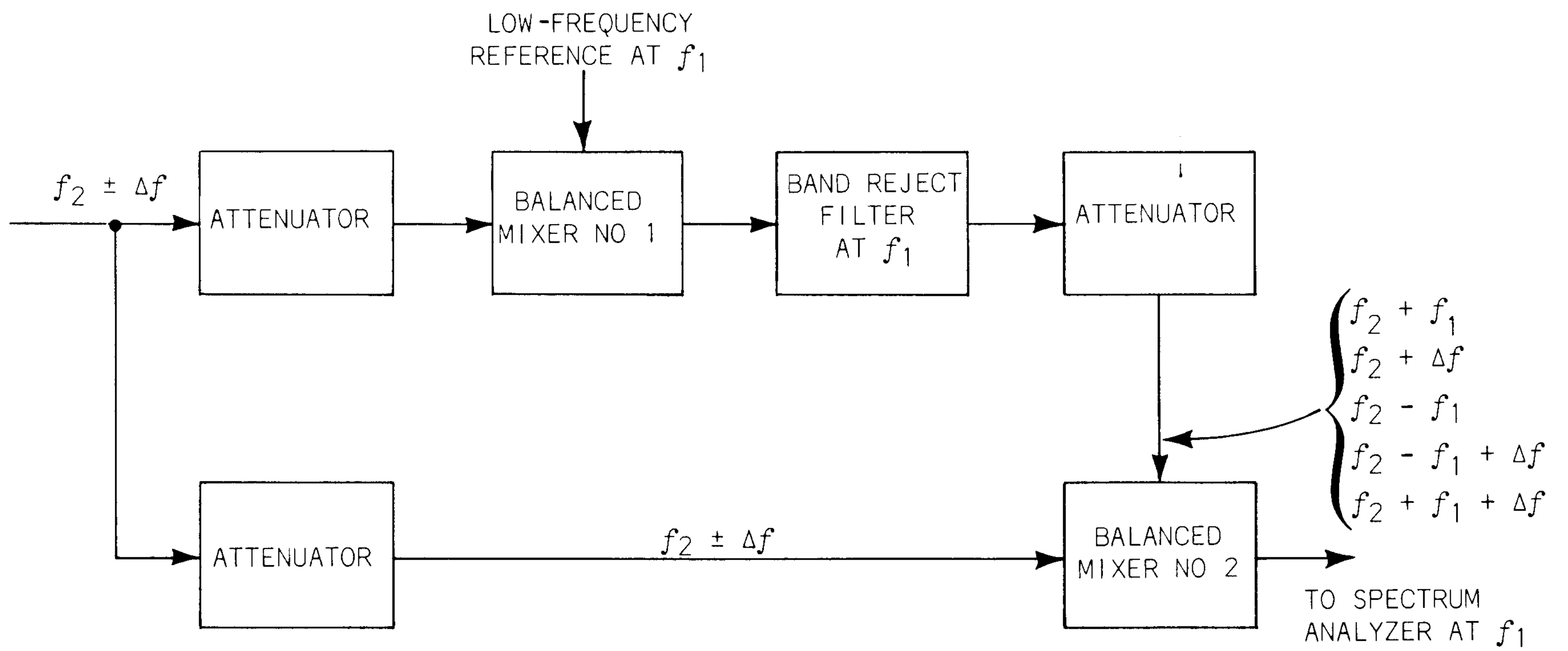
Fig. 6-4. Block diagram of spectral purity measurement.
