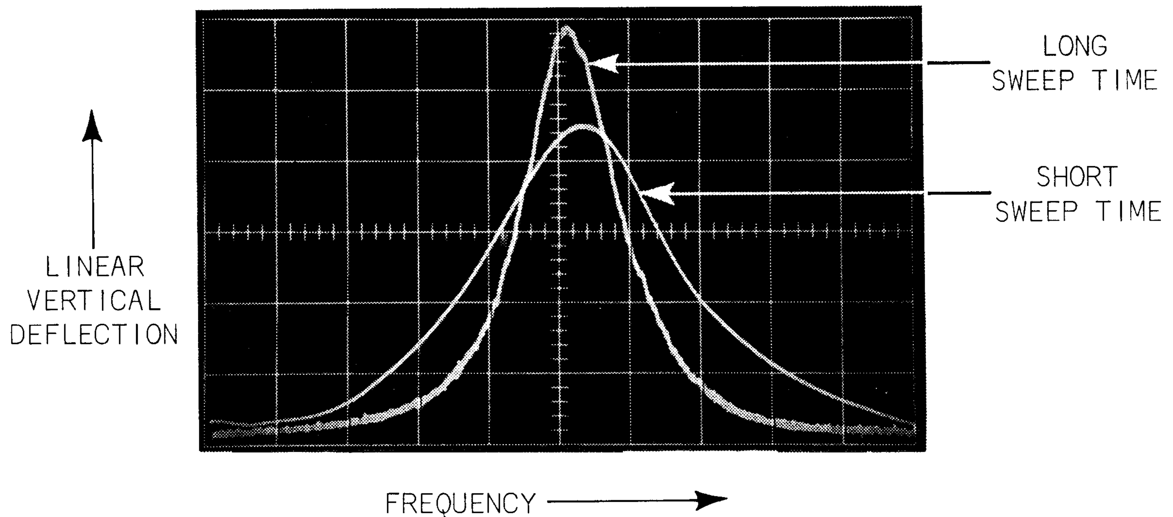
Fig. 3-3. Effect of sweep time on resolution.
