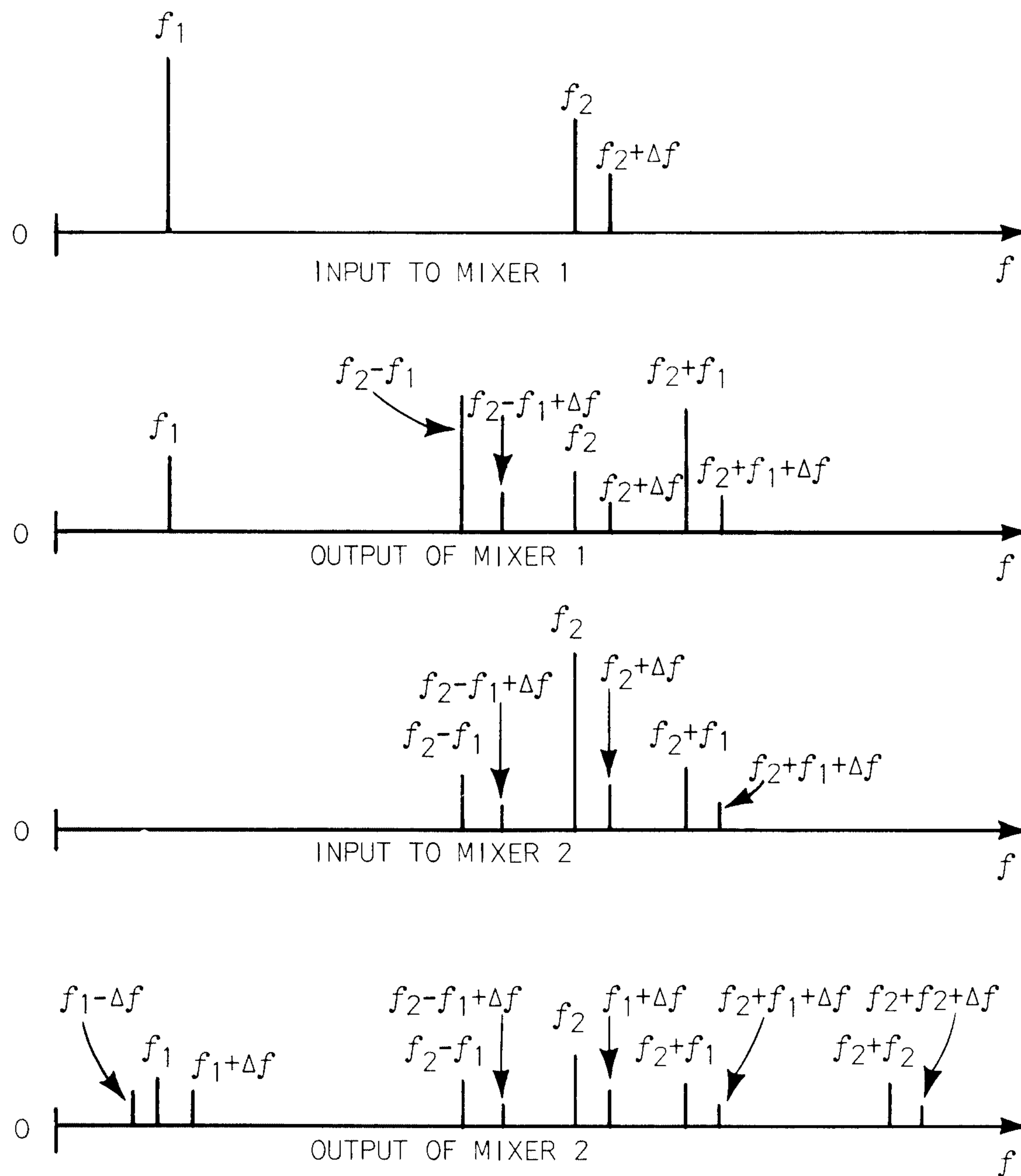
Fig. 6-5. Frequency relationships for the system of Fig. 6-4.
