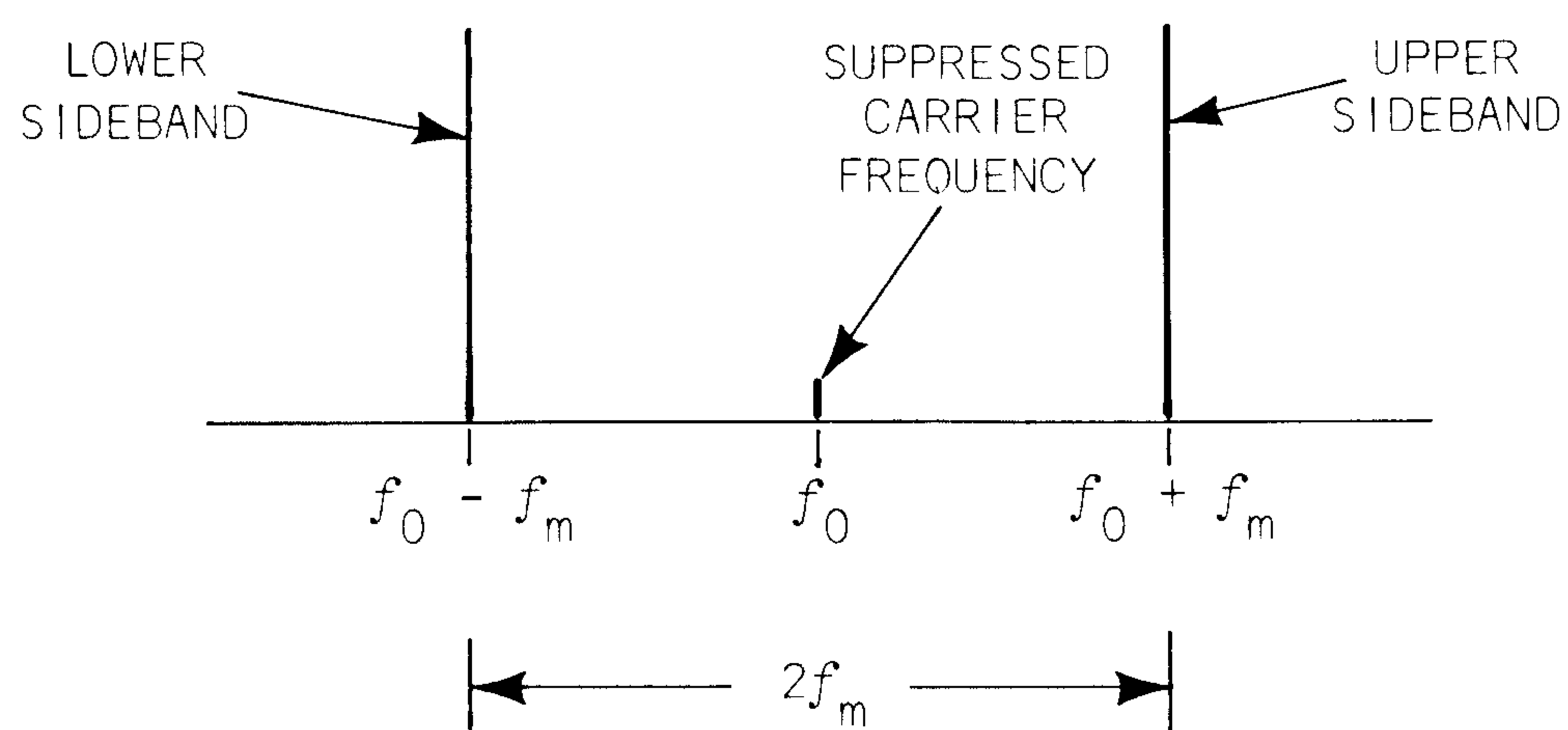
SUPPRESSED CARRIER DOUBLE-SIDEBAND REQUIRES AN RF SPECTRUM EQUAL TO TWICE THE INFORMATION BANDWIDTH.
