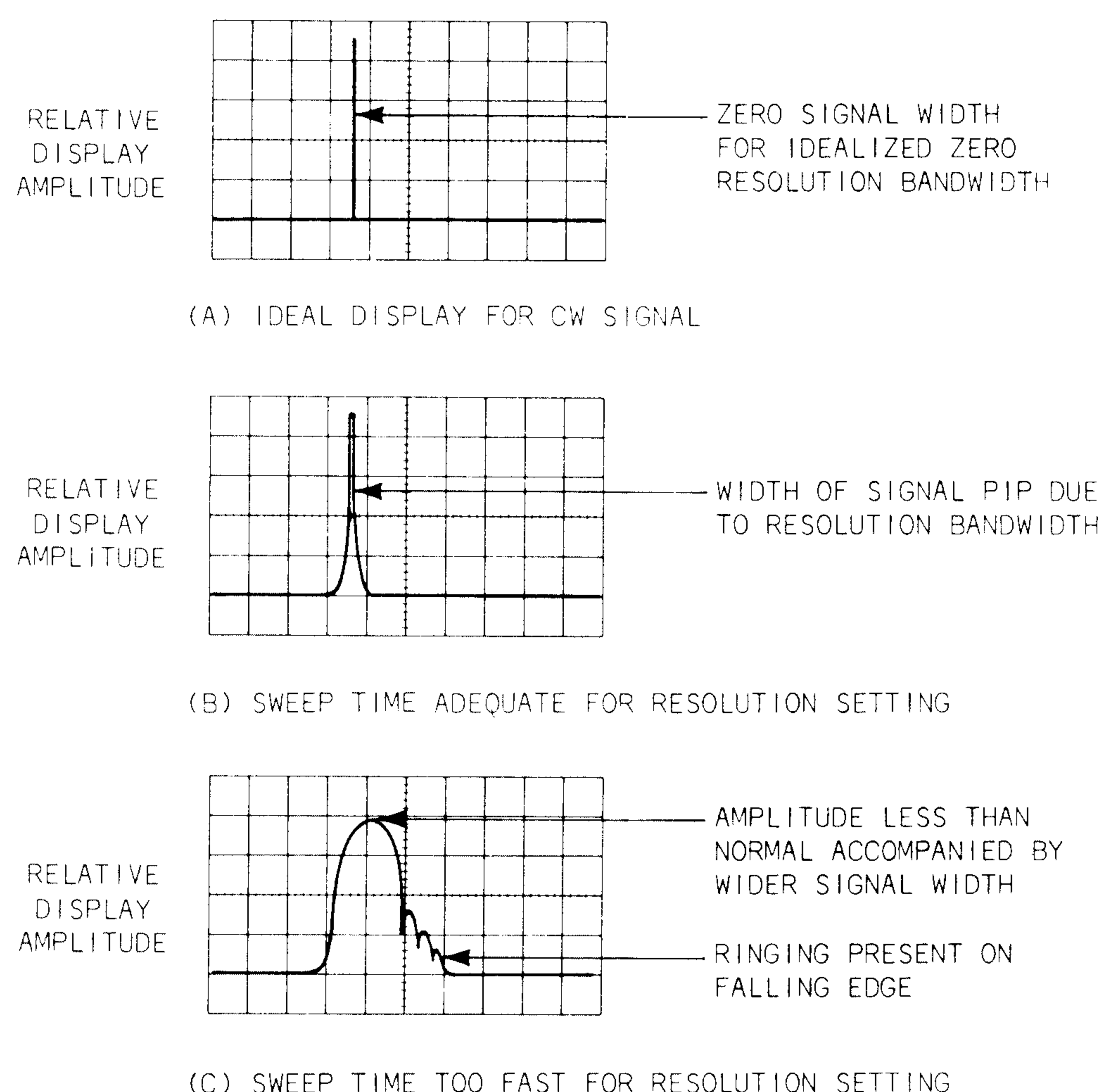
Fig. 4-1. Spectrum analyzer displays.
